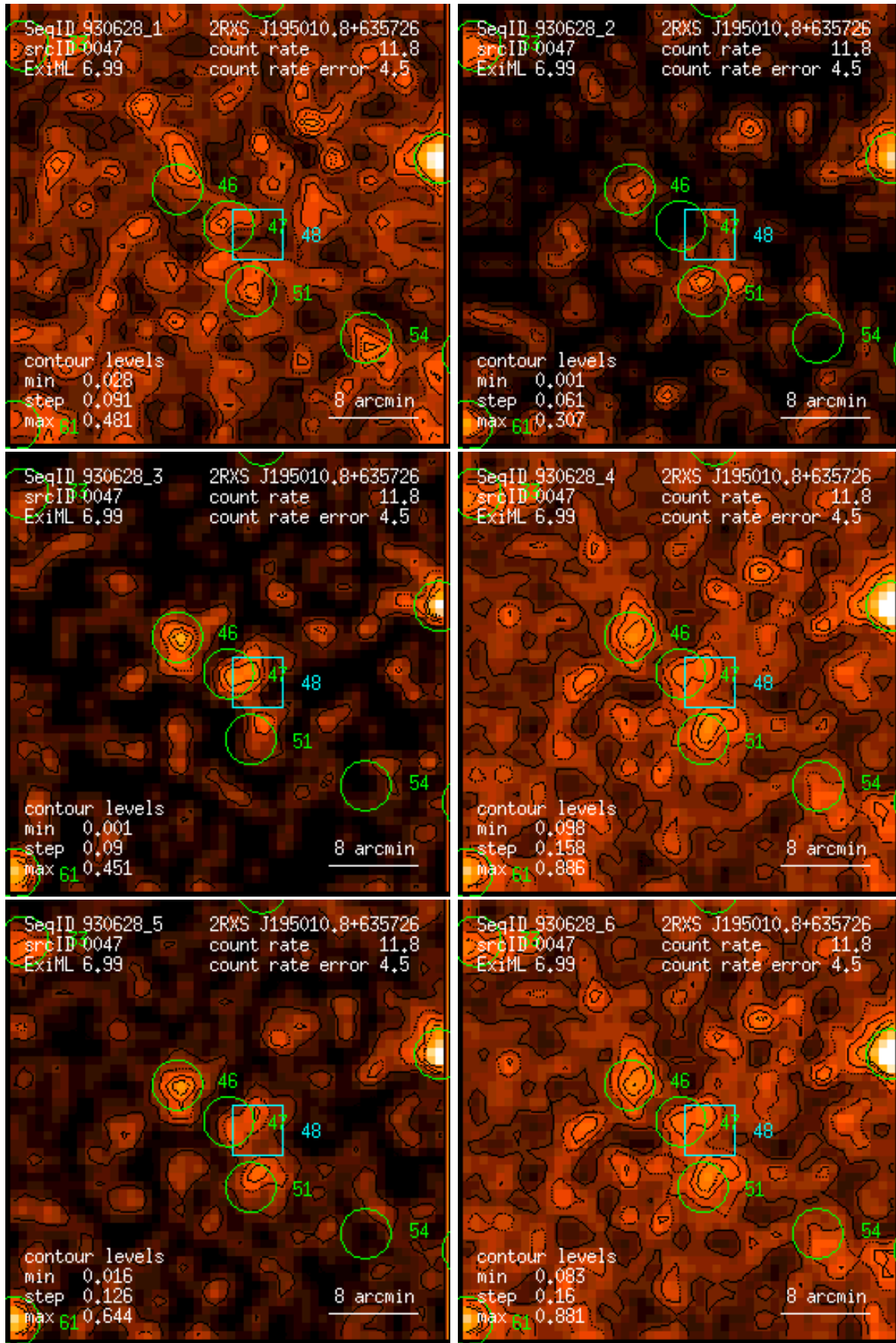
Figure 47: RASS 930628: detection 0047: band rate images, Gaussian filter: (1) PSPC channels 11 – 41, (2) 52 – 90, (3) 91 – 201, (4) 11 – 235, (5) 52 – 201, (6) 11 – 201. Broad band rates in counts/ks. Band rate contour levels in counts/ks/arcmin 2 .
