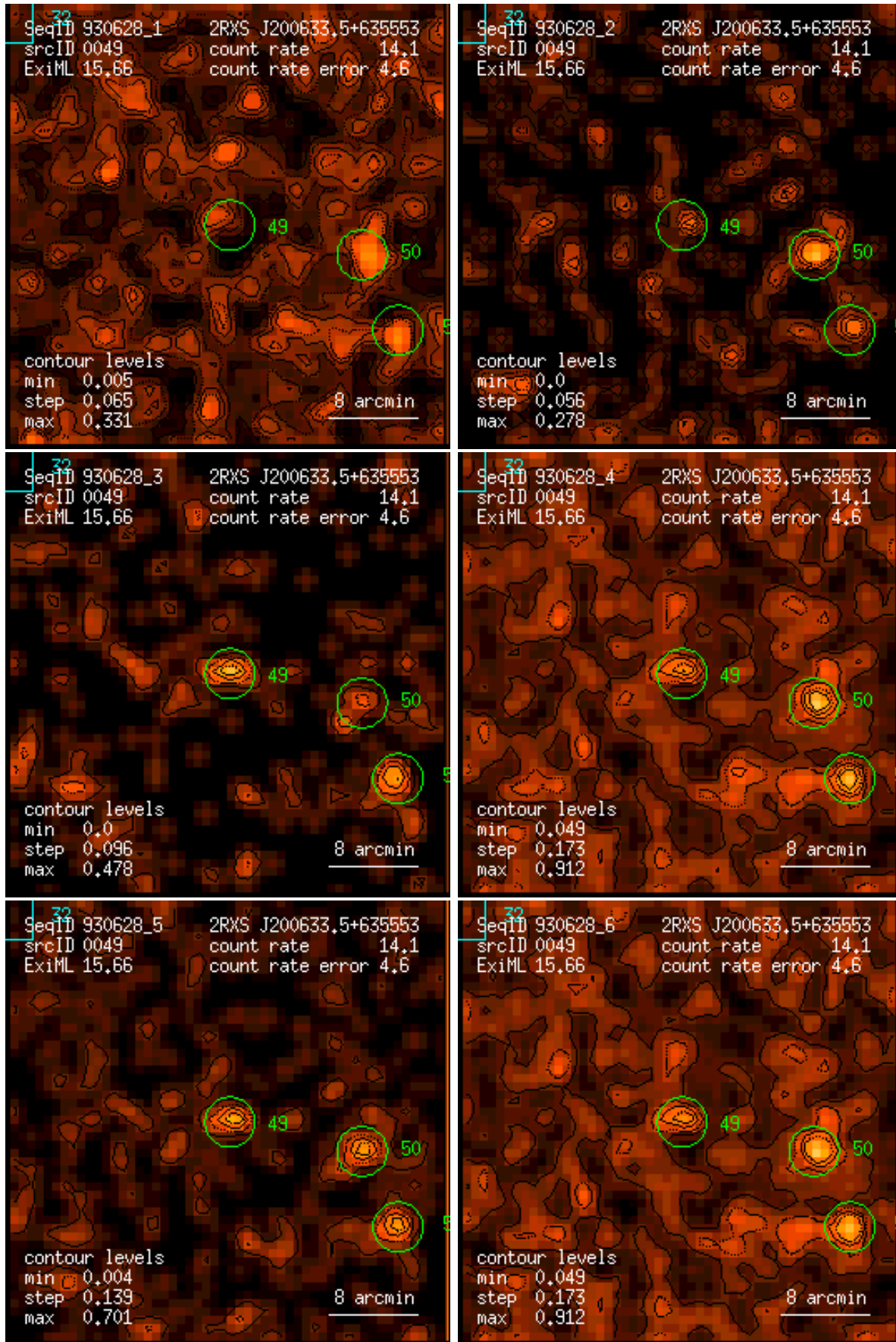
Figure 49: RASS 930628: detection 0049: band rate images, Gaussian filter: (1) PSPC channels 11 – 41, (2) 52 – 90, (3) 91 – 201, (4) 11 – 235, (5) 52 – 201, (6) 11 – 201. Broad band rates in counts/ks. Band rate contour levels in counts/ks/arcmin 2 .
