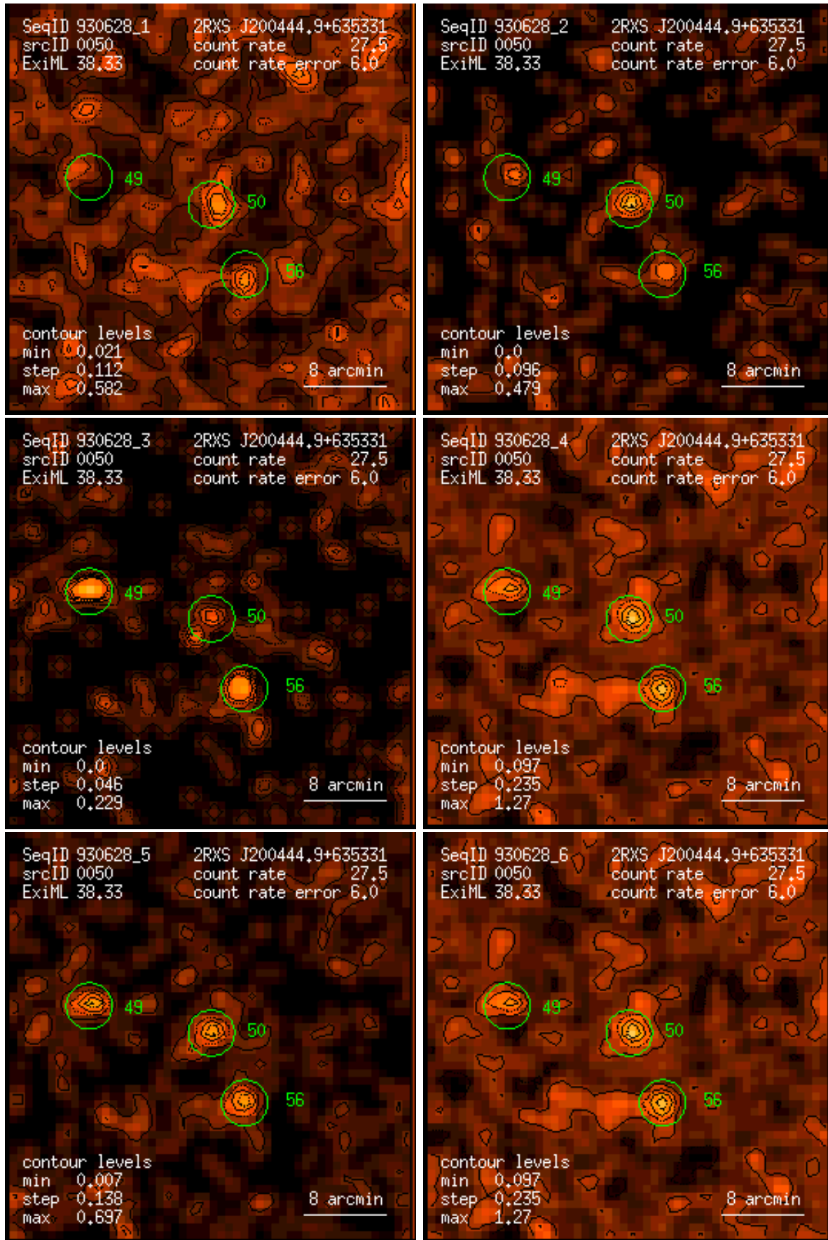
Figure 50: RASS 930628: detection 0050: band rate images, Gaussian filter: (1) PSPC channels 11 – 41, (2) 52 – 90, (3) 91 – 201, (4) 11 – 235, (5) 52 – 201, (6) 11 – 201. Broad band rates in counts/ks. Band rate contour levels in counts/ks/arcmin 2 .
