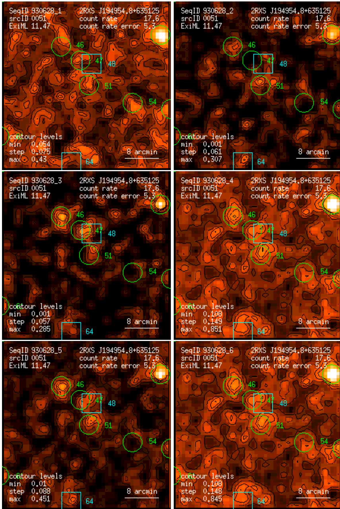
Figure 51: RASS 930628: detection 0051: band rate images, Gaussian filter: (1) PSPC channels 11 – 41, (2) 52 – 90, (3) 91 – 201, (4) 11 – 235, (5) 52 – 201, (6) 11 – 201. Broad band rates in counts/ks. Band rate contour levels in counts/ks/arcmin 2 .
