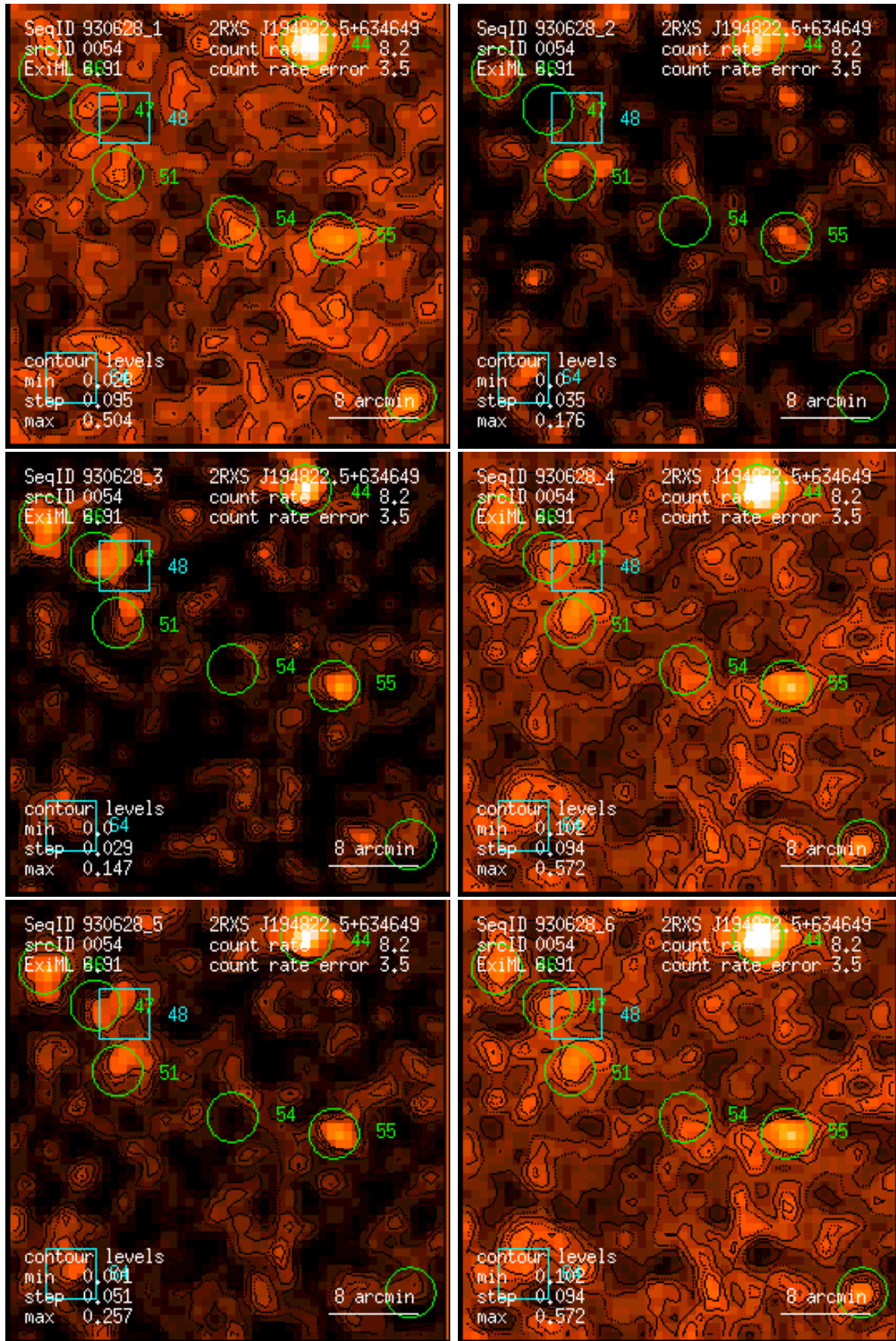
Figure 54: RASS 930628: detection 0054: band rate images, Gaussian filter: (1) PSPC channels 11 – 41, (2) 52 – 90, (3) 91 – 201, (4) 11 – 235, (5) 52 – 201, (6) 11 – 201. Broad band rates in counts/ks. Band rate contour levels in counts/ks/arcmin 2 .
