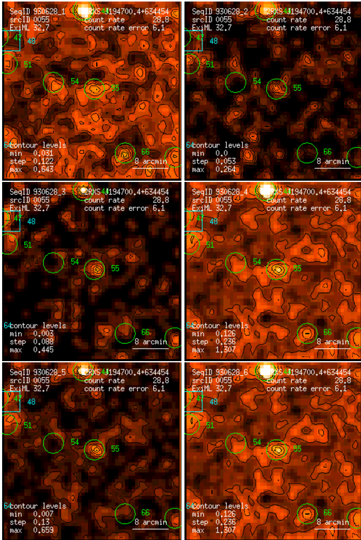
Figure 55: RASS 930628: detection 0055: band rate images, Gaussian filter: (1) PSPC channels 11 – 41, (2) 52 – 90, (3) 91 – 201, (4) 11 – 235, (5) 52 – 201, (6) 11 – 201. Broad band rates in counts/ks. Band rate contour levels in counts/ks/arcmin 2 .
