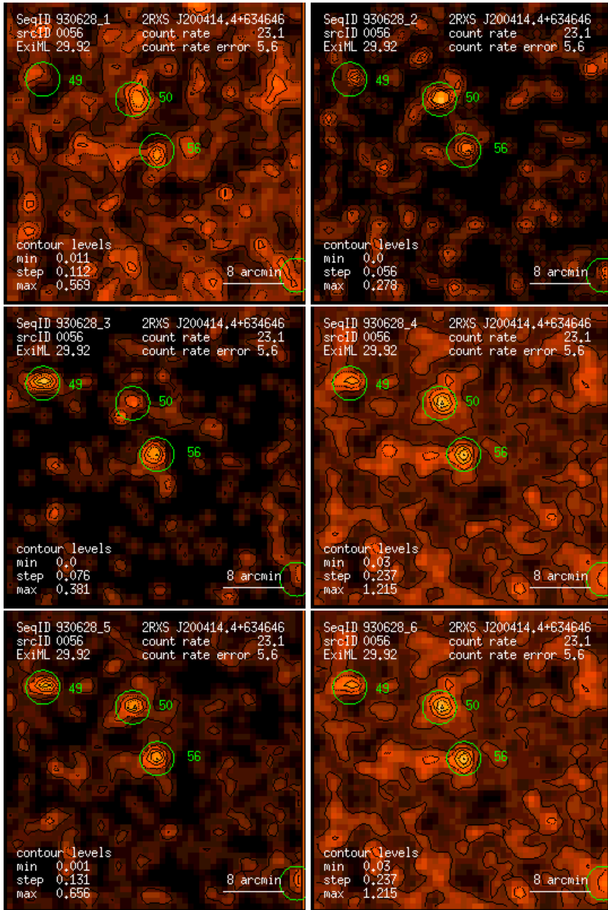
Figure 56: RASS 930628: detection 0056: band rate images, Gaussian filter: (1) PSPC channels 11 – 41, (2) 52 – 90, (3) 91 – 201, (4) 11 – 235, (5) 52 – 201, (6) 11 – 201. Broad band rates in counts/ks. Band rate contour levels in counts/ks/arcmin 2 .
