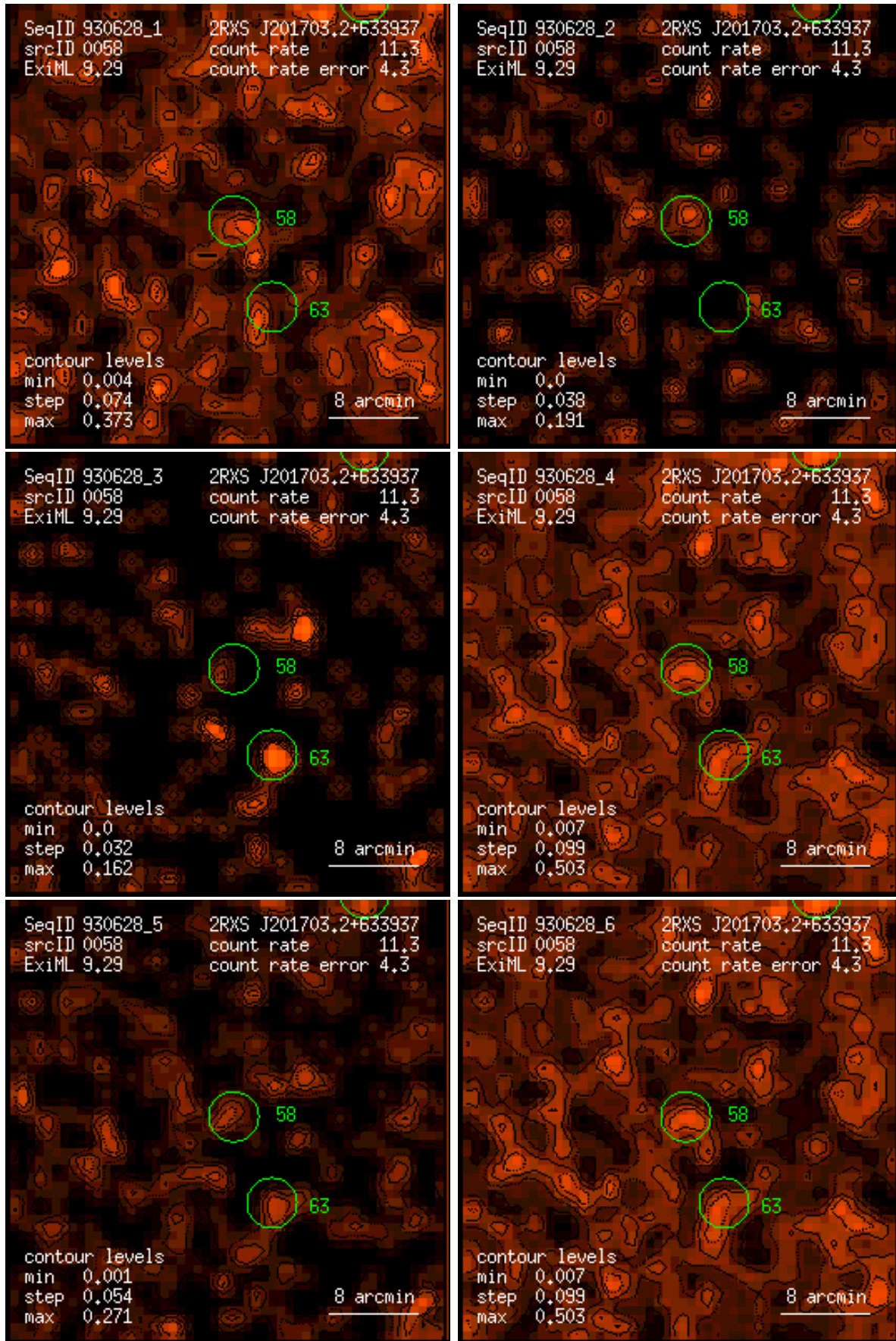
Figure 58: RASS 930628: detection 0058: band rate images, Gaussian filter: (1) PSPC channels 11 – 41, (2) 52 – 90, (3) 91 – 201, (4) 11 – 235, (5) 52 – 201, (6) 11 – 201. Broad band rates in counts/ks. Band rate contour levels in counts/ks/arcmin 2 .
