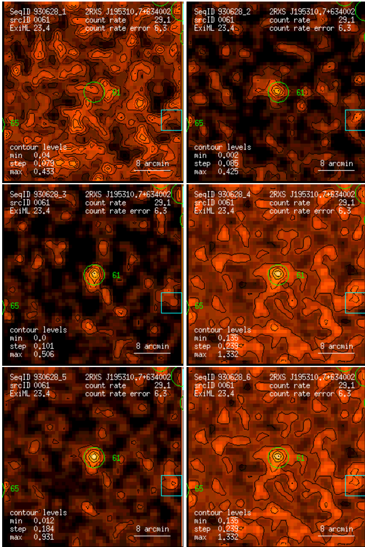
Figure 61: RASS 930628: detection 0061: band rate images, Gaussian filter: (1) PSPC channels 11 – 41, (2) 52 – 90, (3) 91 – 201, (4) 11 – 235, (5) 52 – 201, (6) 11 – 201. Broad band rates in counts/ks. Band rate contour levels in counts/ks/arcmin 2 .
