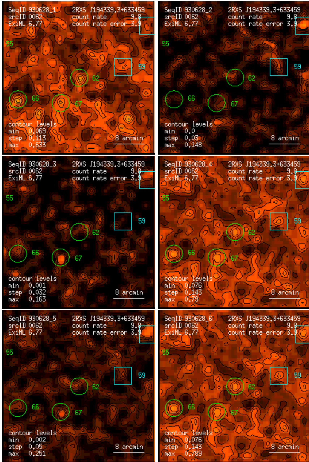
Figure 62: RASS 930628: detection 0062: band rate images, Gaussian filter: (1) PSPC channels 11 – 41, (2) 52 – 90, (3) 91 – 201, (4) 11 – 235, (5) 52 – 201, (6) 11 – 201. Broad band rates in counts/ks. Band rate contour levels in counts/ks/arcmin 2 .
