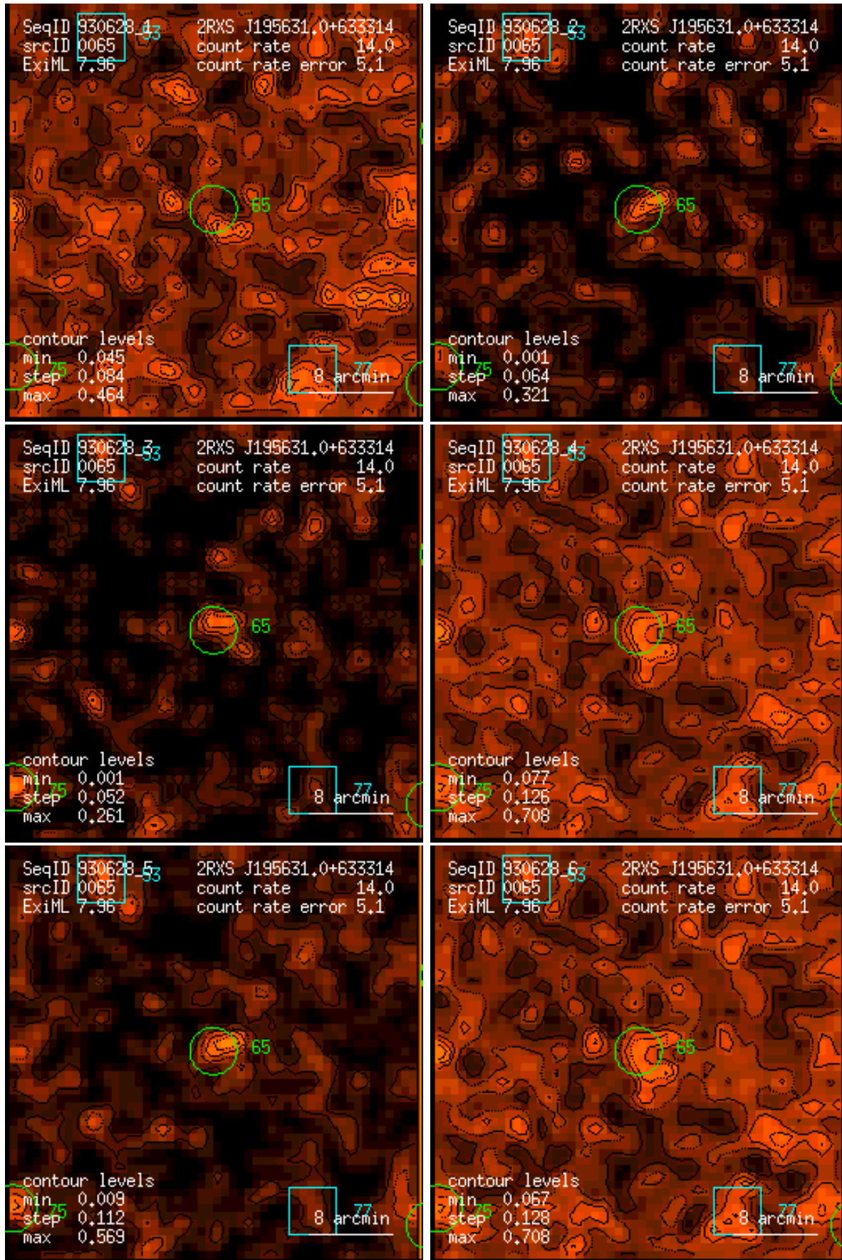
Figure 65: RASS 930628: detection 0065: band rate images, Gaussian filter: (1) PSPC channels 11 – 41, (2) 52 – 90, (3) 91 – 201, (4) 11 – 235, (5) 52 – 201, (6) 11 – 201. Broad band rates in counts/ks. Band rate contour levels in counts/ks/arcmin 2 .
