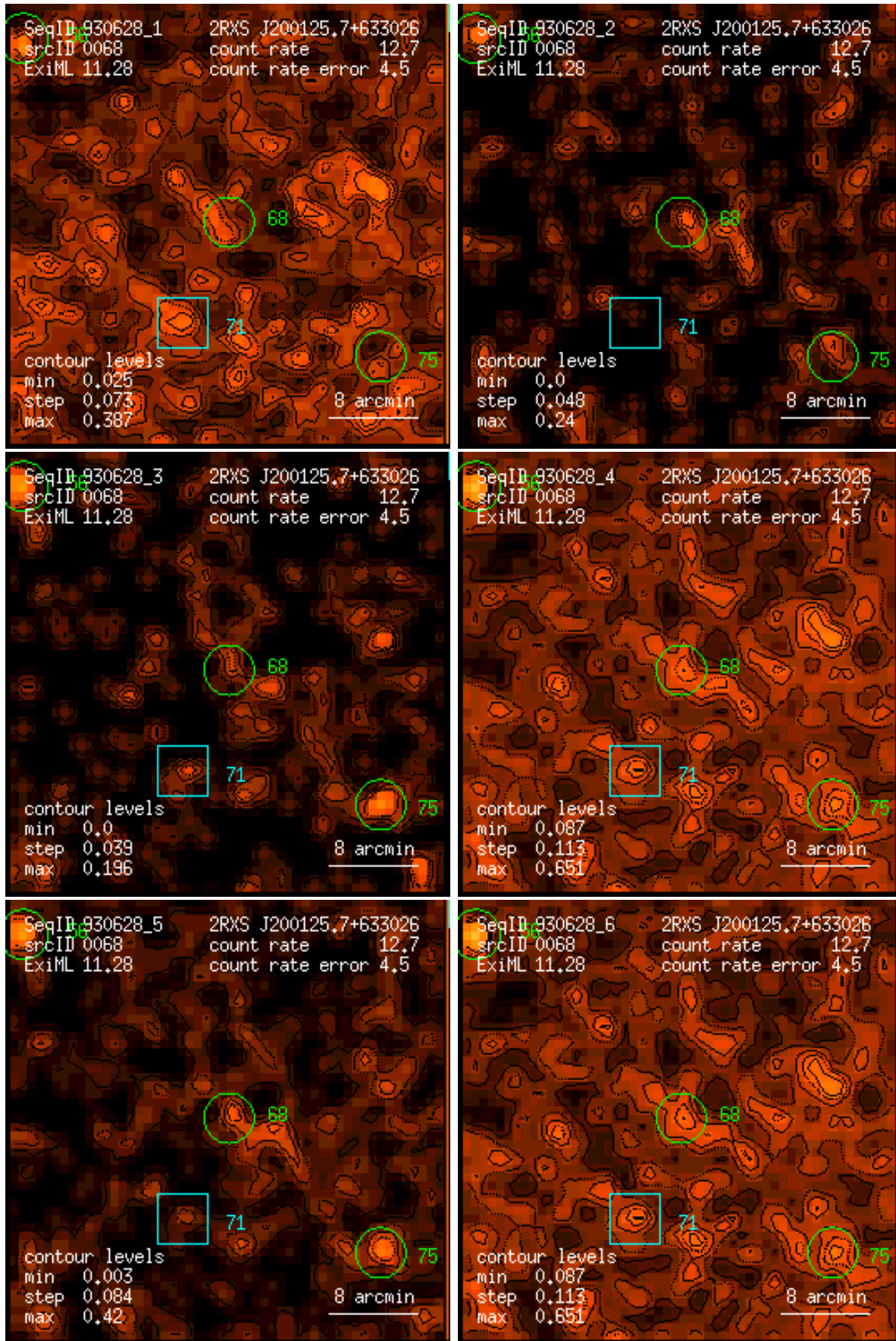
Figure 68: RASS 930628: detection 0068: band rate images, Gaussian filter: (1) PSPC channels 11 – 41, (2) 52 – 90, (3) 91 – 201, (4) 11 – 235, (5) 52 – 201, (6) 11 – 201. Broad band rates in counts/ks. Band rate contour levels in counts/ks/arcmin 2 .
