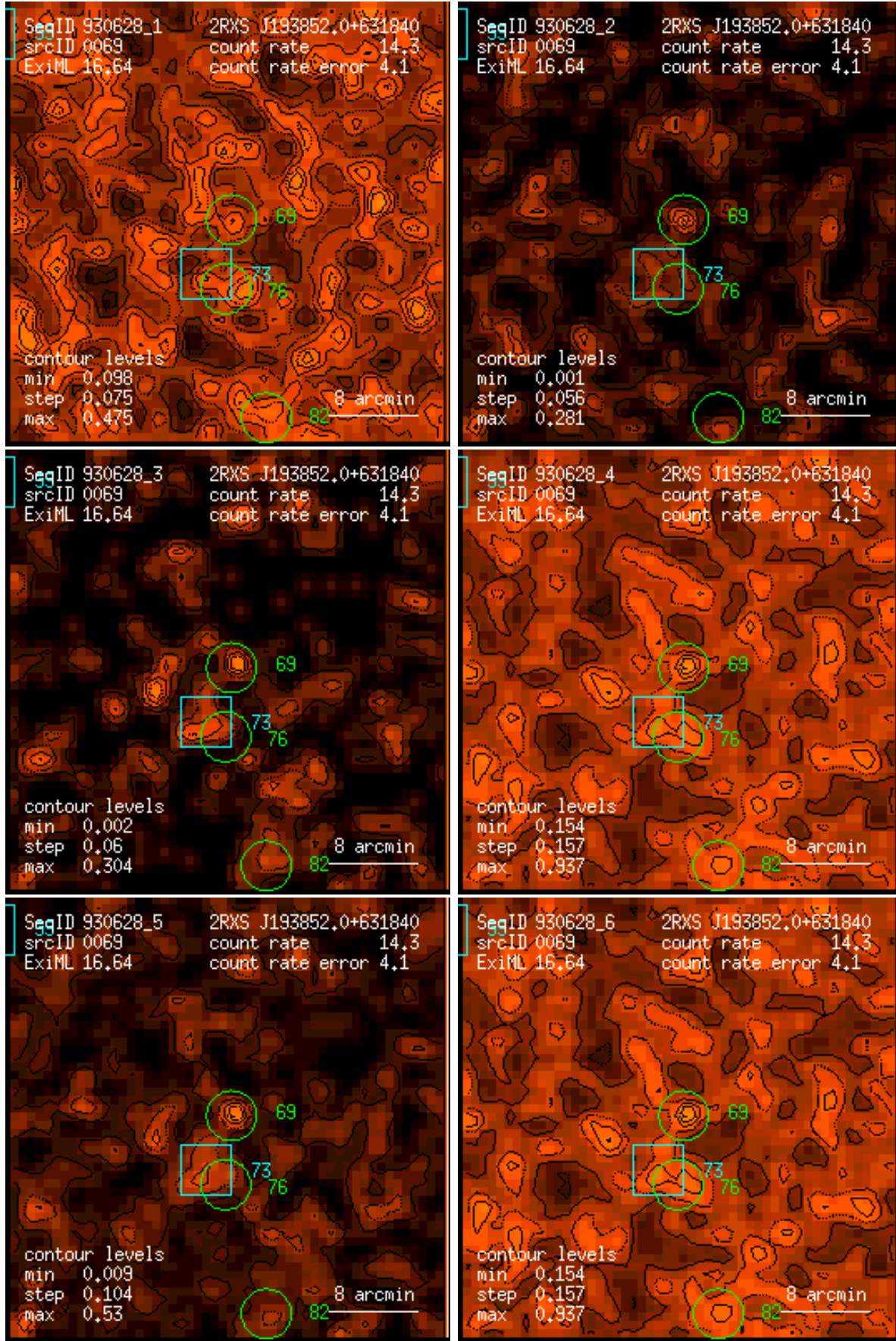
Figure 69: RASS 930628: detection 0069: band rate images, Gaussian filter: (1) PSPC channels 11 – 41, (2) 52 – 90, (3) 91 – 201, (4) 11 – 235, (5) 52 – 201, (6) 11 – 201. Broad band rates in counts/ks. Band rate contour levels in counts/ks/arcmin 2 .
