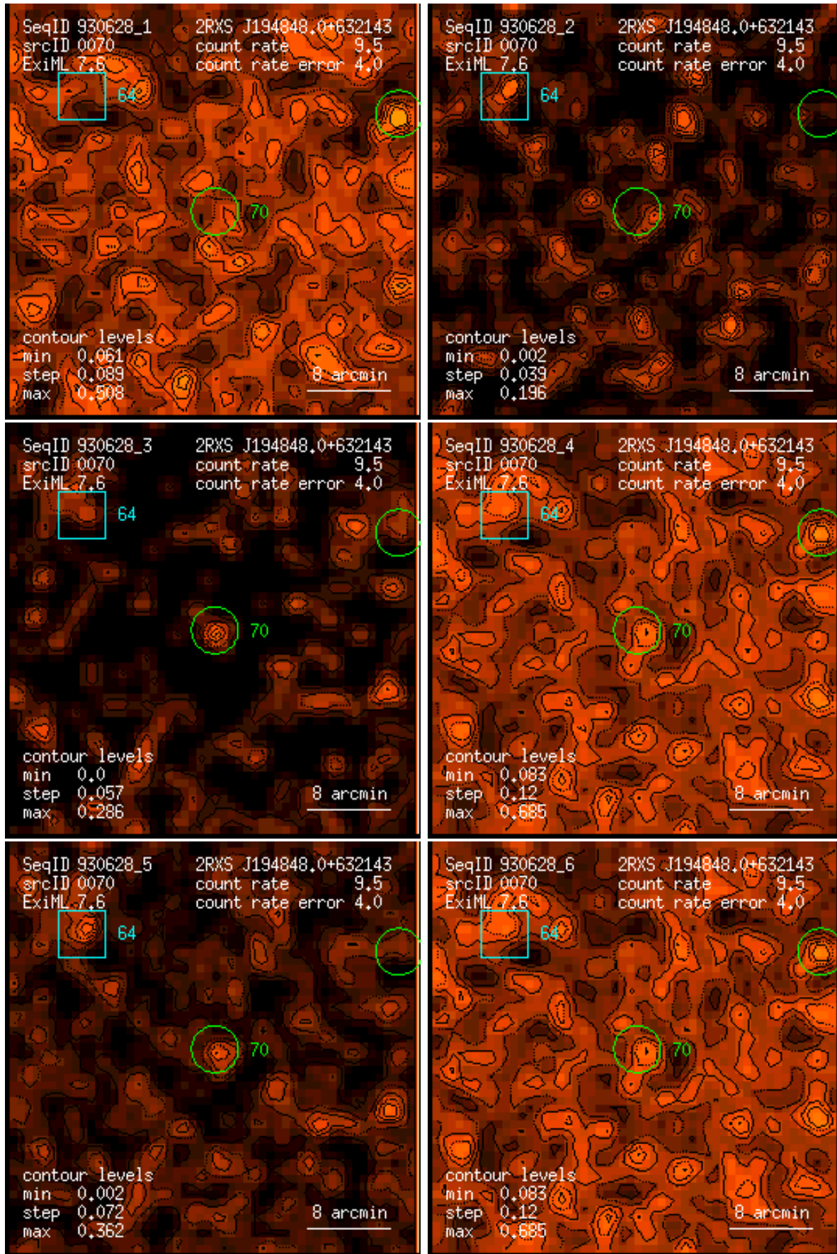
Figure 70: RASS 930628: detection 0070: band rate images, Gaussian filter: (1) PSPC channels 11 – 41, (2) 52 – 90, (3) 91 – 201, (4) 11 – 235, (5) 52 – 201, (6) 11 – 201. Broad band rates in counts/ks. Band rate contour levels in counts/ks/arcmin 2 .
