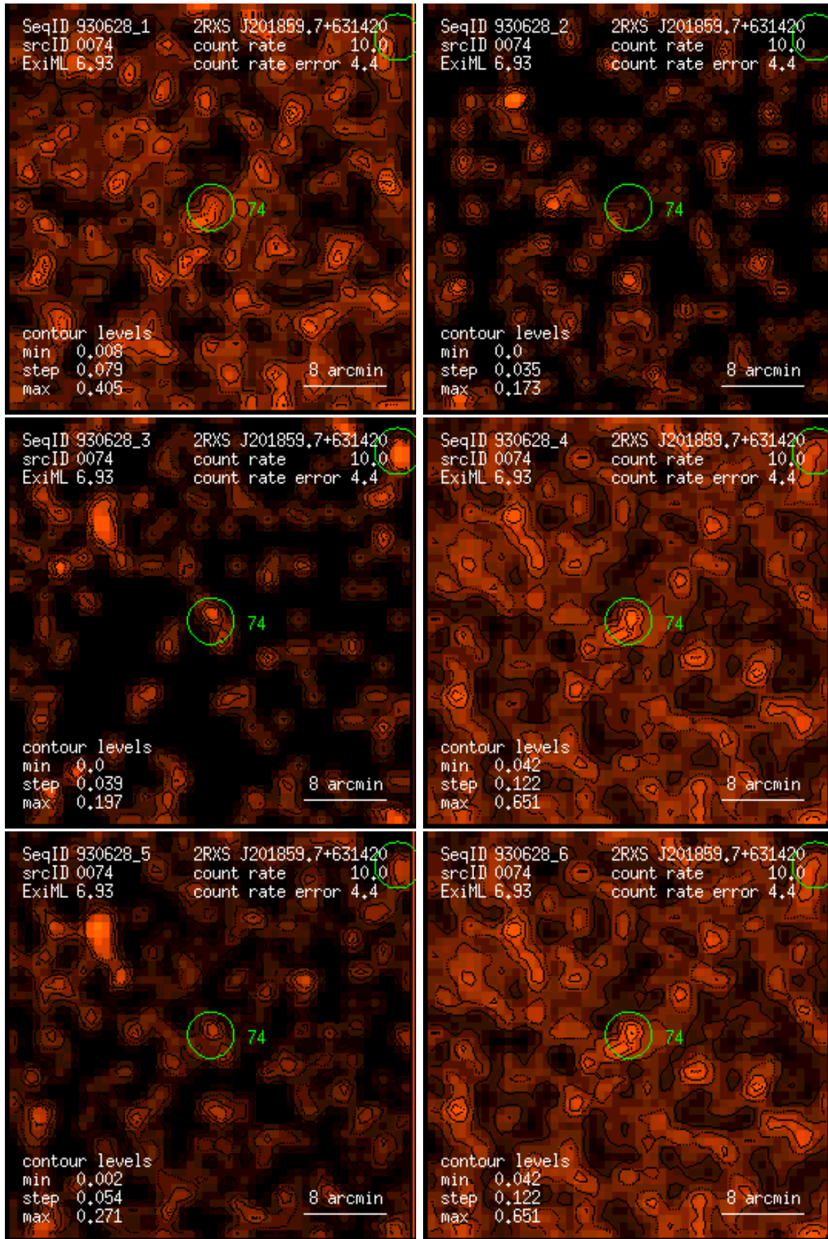
Figure 74: RASS 930628: detection 0074: band rate images, Gaussian filter: (1) PSPC channels 11 – 41, (2) 52 – 90, (3) 91 – 201, (4) 11 – 235, (5) 52 – 201, (6) 11 – 201. Broad band rates in counts/ks. Band rate contour levels in counts/ks/arcmin 2 .
