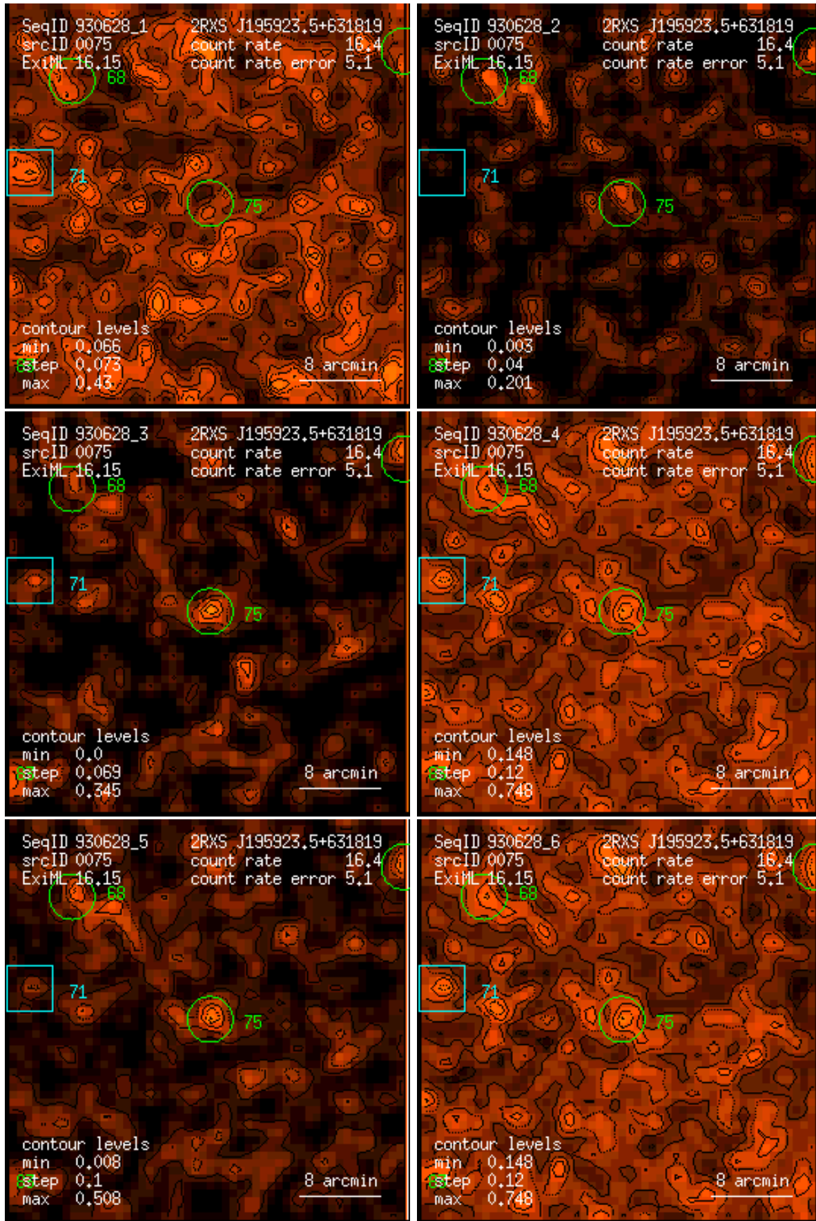
Figure 75: RASS 930628: detection 0075: band rate images, Gaussian filter: (1) PSPC channels 11 – 41, (2) 52 – 90, (3) 91 – 201, (4) 11 – 235, (5) 52 – 201, (6) 11 – 201. Broad band rates in counts/ks. Band rate contour levels in counts/ks/arcmin 2 .
