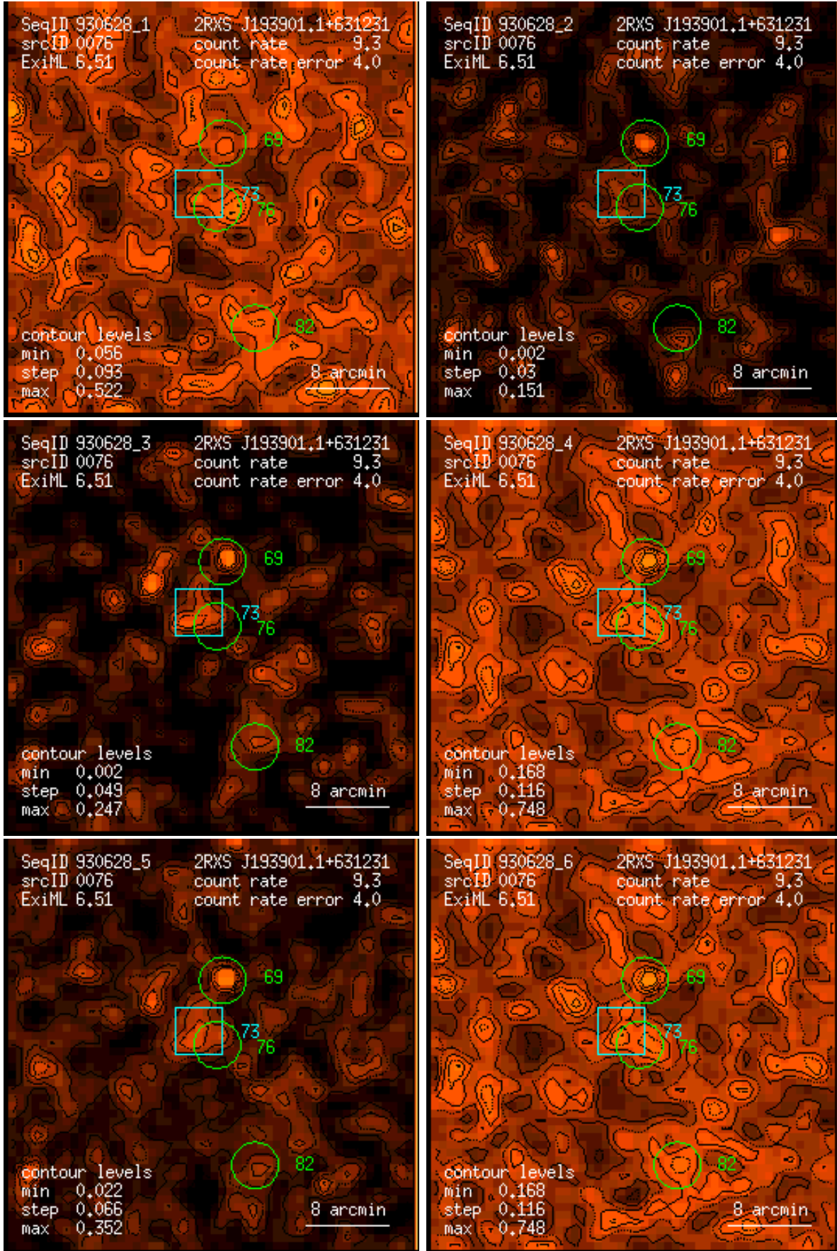
Figure 76: RASS 930628: detection 0076: band rate images, Gaussian filter: (1) PSPC channels 11 – 41, (2) 52 – 90, (3) 91 – 201, (4) 11 – 235, (5) 52 – 201, (6) 11 – 201. Broad band rates in counts/ks. Band rate contour levels in counts/ks/arcmin 2 .
