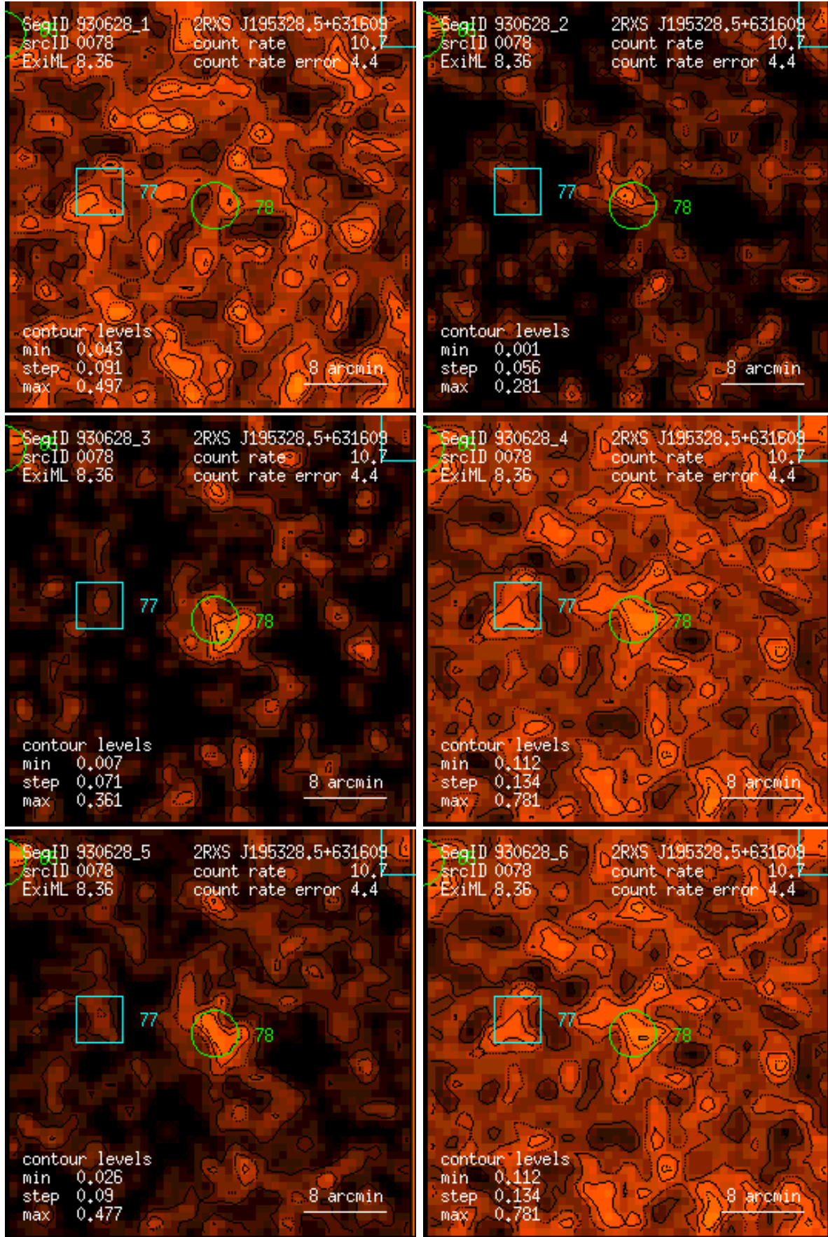
Figure 78: RASS 930628: detection 0078: band rate images, Gaussian filter: (1) PSPC channels 11 – 41, (2) 52 – 90, (3) 91 – 201, (4) 11 – 235, (5) 52 – 201, (6) 11 – 201. Broad band rates in counts/ks. Band rate contour levels in counts/ks/arcmin 2 .
