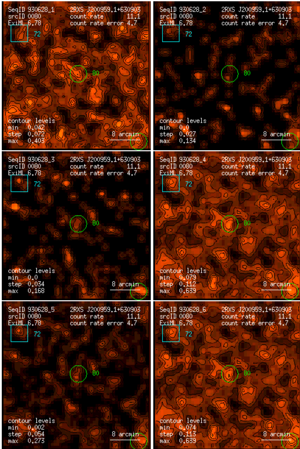
Figure 80: RASS 930628: detection 0080: band rate images, Gaussian filter: (1) PSPC channels 11 – 41, (2) 52 – 90, (3) 91 – 201, (4) 11 – 235, (5) 52 – 201, (6) 11 – 201. Broad band rates in counts/ks. Band rate contour levels in counts/ks/arcmin 2 .
