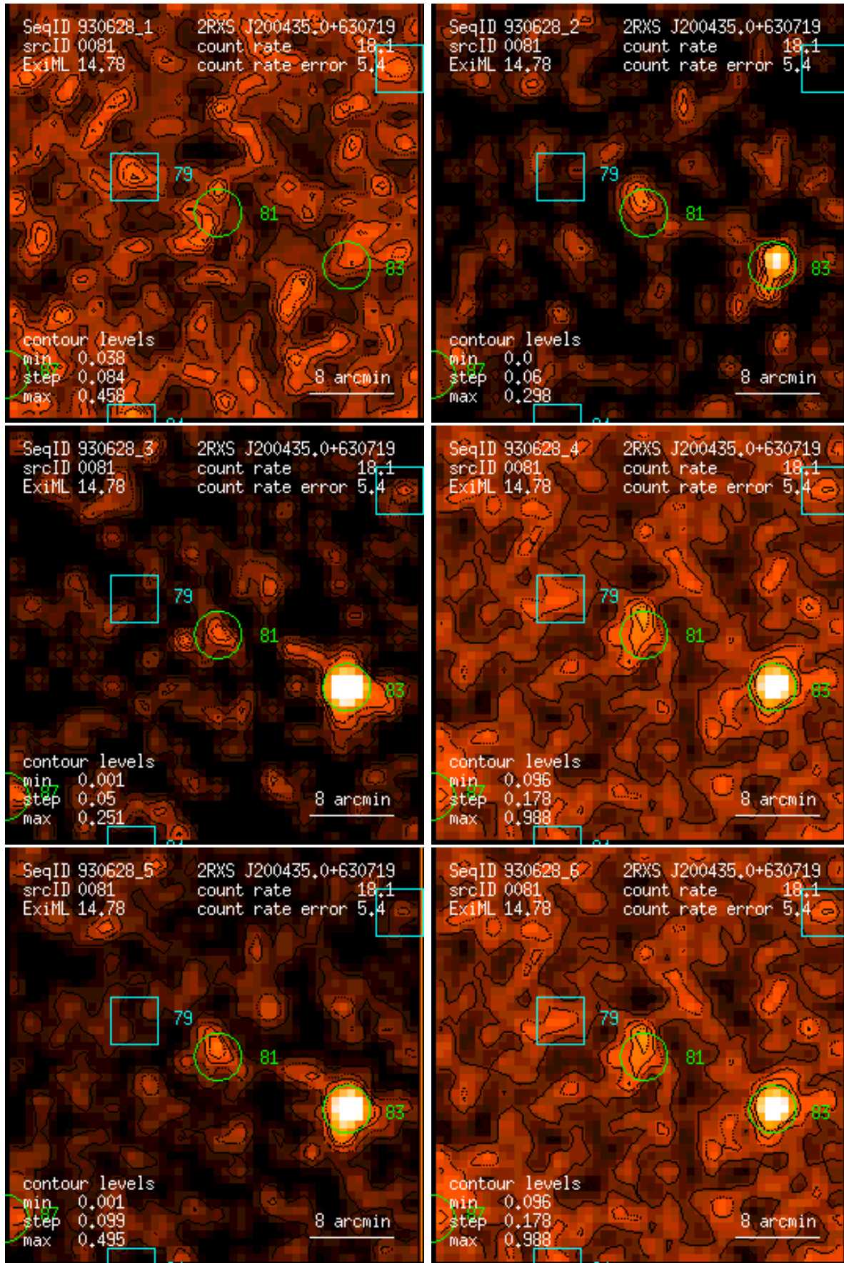
Figure 81: RASS 930628: detection 0081: band rate images, Gaussian filter: (1) PSPC channels 11 – 41, (2) 52 – 90, (3) 91 – 201, (4) 11 – 235, (5) 52 – 201, (6) 11 – 201. Broad band rates in counts/ks. Band rate contour levels in counts/ks/arcmin 2 .
