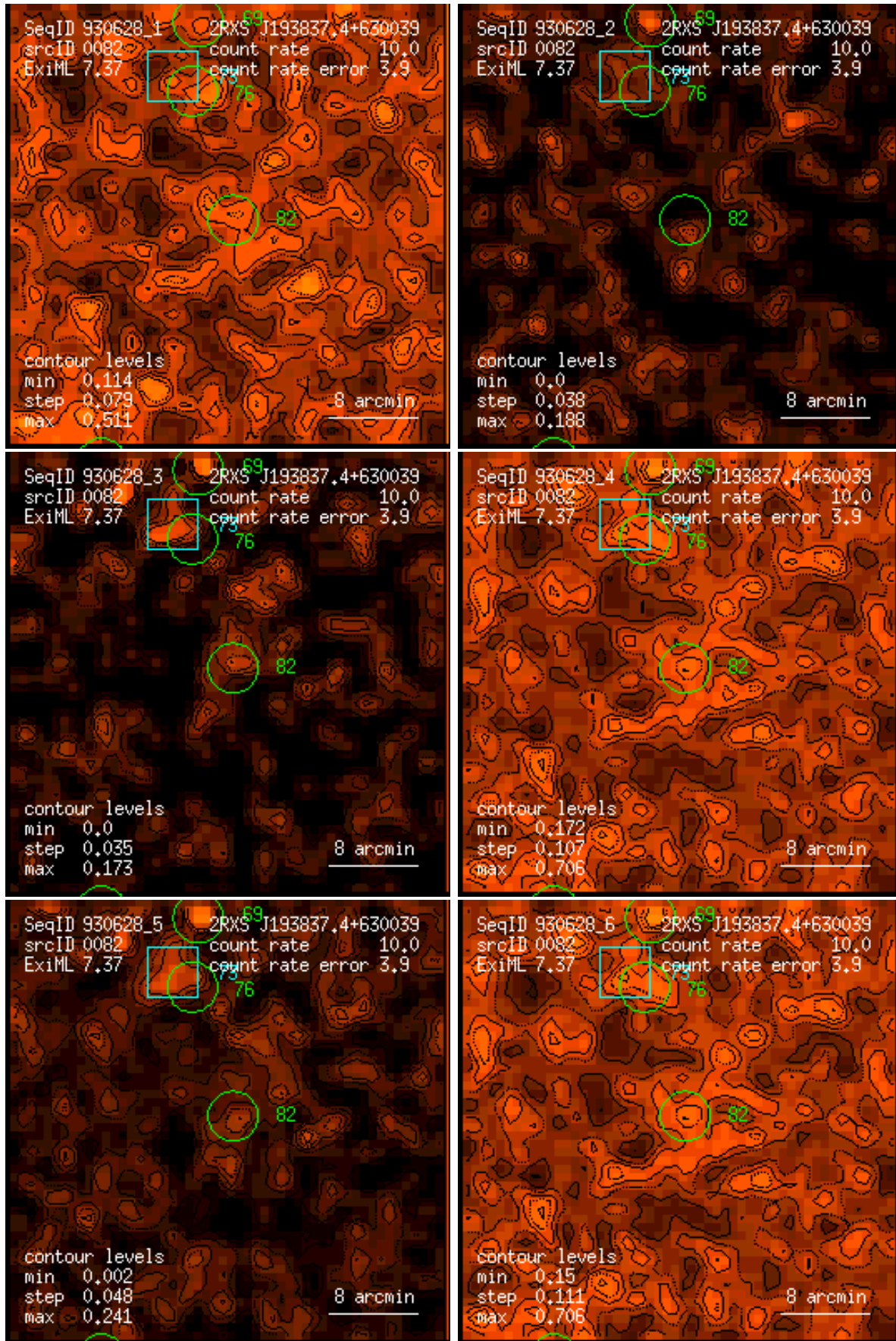
Figure 82: RASS 930628: detection 0082: band rate images, Gaussian filter: (1) PSPC channels 11 – 41, (2) 52 – 90, (3) 91 – 201, (4) 11 – 235, (5) 52 – 201, (6) 11 – 201. Broad band rates in counts/ks. Band rate contour levels in counts/ks/arcmin 2 .
