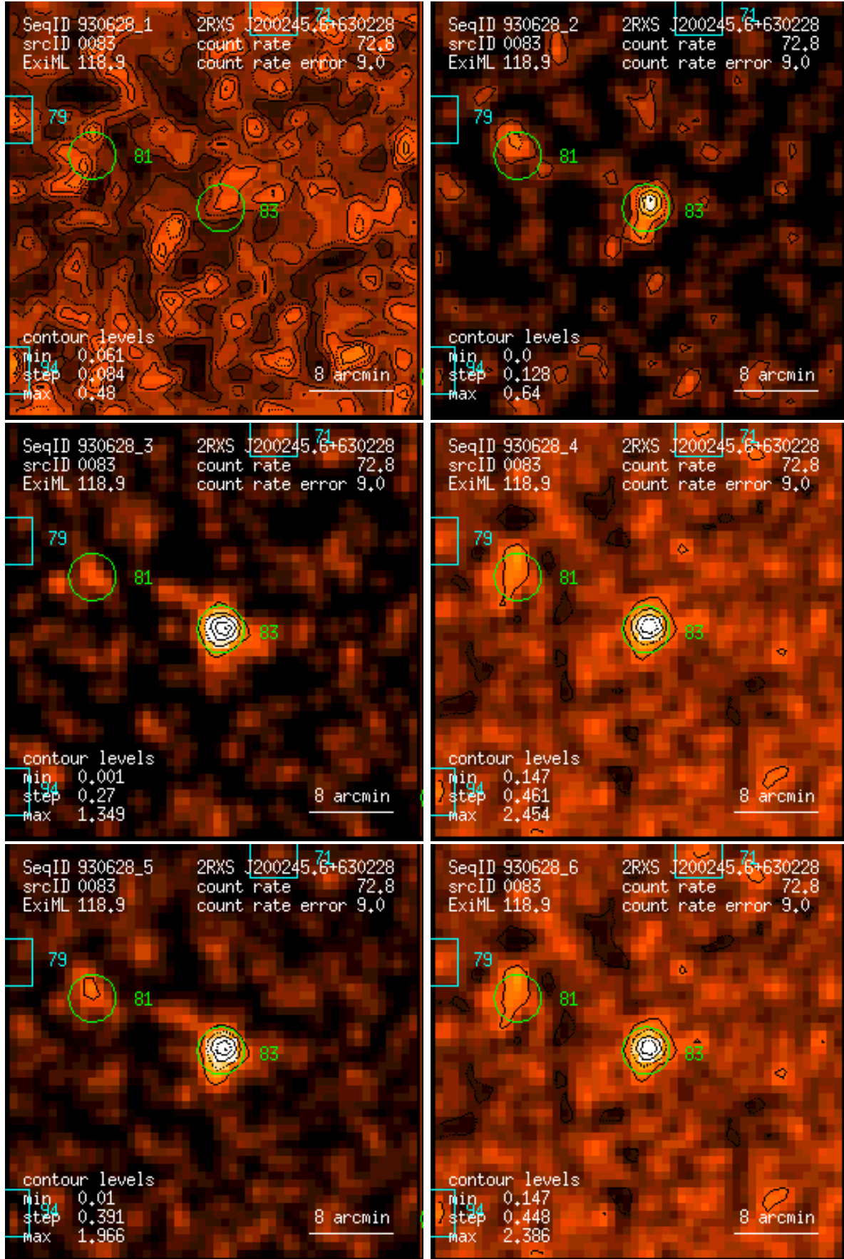
Figure 83: RASS 930628: detection 0083: band rate images, Gaussian filter: (1) PSPC channels 11 – 41, (2) 52 – 90, (3) 91 – 201, (4) 11 – 235, (5) 52 – 201, (6) 11 – 201. Broad band rates in counts/ks. Band rate contour levels in counts/ks/arcmin 2 .
