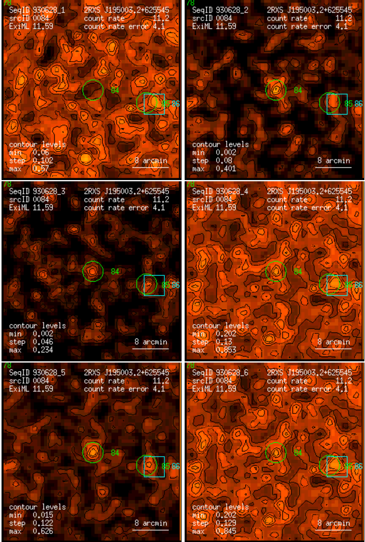
Figure 84: RASS 930628: detection 0084: band rate images, Gaussian filter: (1) PSPC channels 11 – 41, (2) 52 – 90, (3) 91 – 201, (4) 11 – 235, (5) 52 – 201, (6) 11 – 201. Broad band rates in counts/ks. Band rate contour levels in counts/ks/arcmin 2 .
