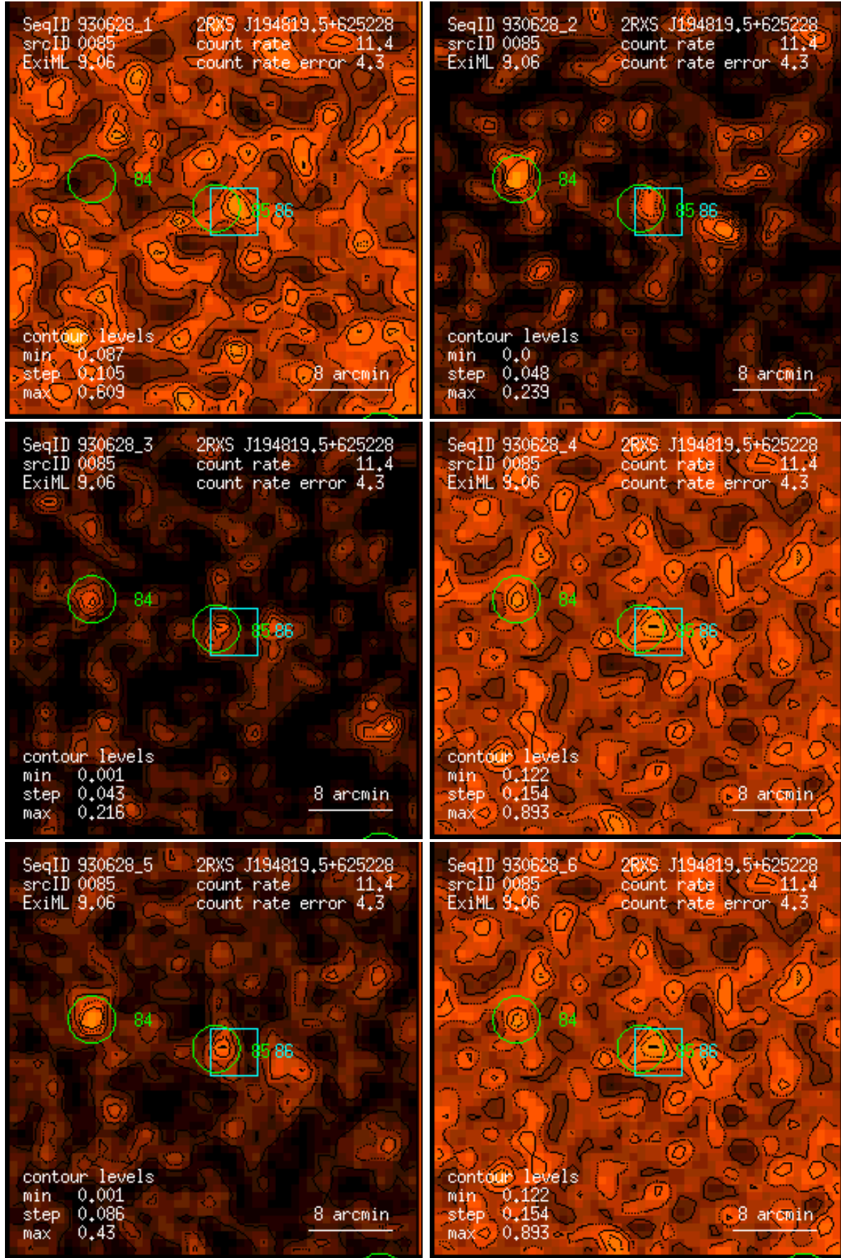
Figure 85: RASS 930628: detection 0085: band rate images, Gaussian filter: (1) PSPC channels 11 – 41, (2) 52 – 90, (3) 91 – 201, (4) 11 – 235, (5) 52 – 201, (6) 11 – 201. Broad band rates in counts/ks. Band rate contour levels in counts/ks/arcmin 2 .
