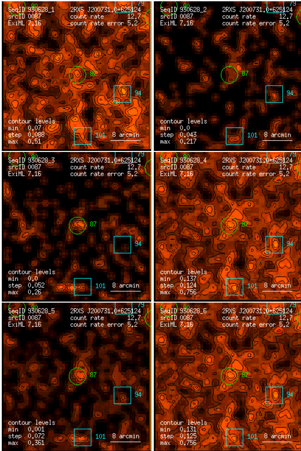
Figure 87: RASS 930628: detection 0087: band rate images, Gaussian filter: (1) PSPC channels 11 – 41, (2) 52 – 90, (3) 91 – 201, (4) 11 – 235, (5) 52 – 201, (6) 11 – 201. Broad band rates in counts/ks. Band rate contour levels in counts/ks/arcmin 2 .
