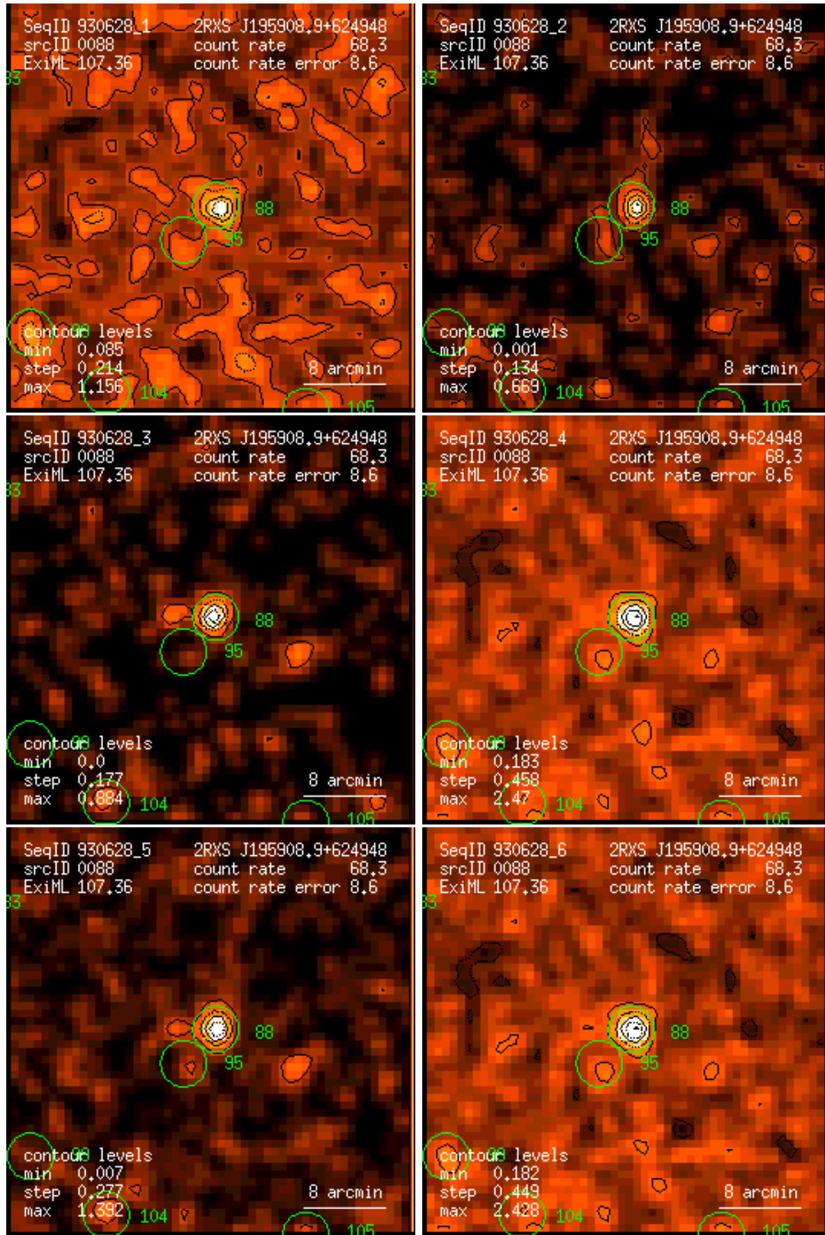
Figure 88: RASS 930628: detection 0088: band rate images, Gaussian filter: (1) PSPC channels 11 – 41, (2) 52 – 90, (3) 91 – 201, (4) 11 – 235, (5) 52 – 201, (6) 11 – 201. Broad band rates in counts/ks. Band rate contour levels in counts/ks/arcmin 2 .
