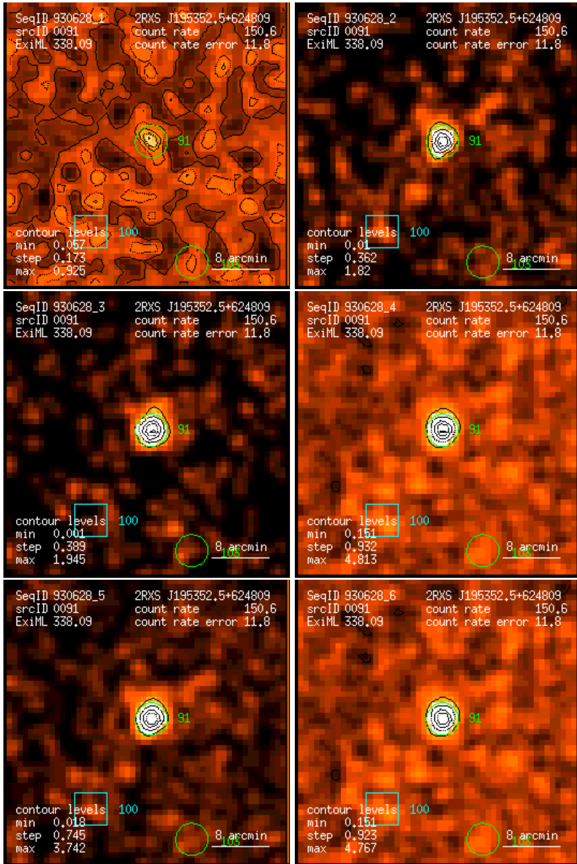
Figure 91: RASS 930628: detection 0091: band rate images, Gaussian filter: (1) PSPC channels 11 – 41, (2) 52 – 90, (3) 91 – 201, (4) 11 – 235, (5) 52 – 201, (6) 11 – 201. Broad band rates in counts/ks. Band rate contour levels in counts/ks/arcmin 2 .
