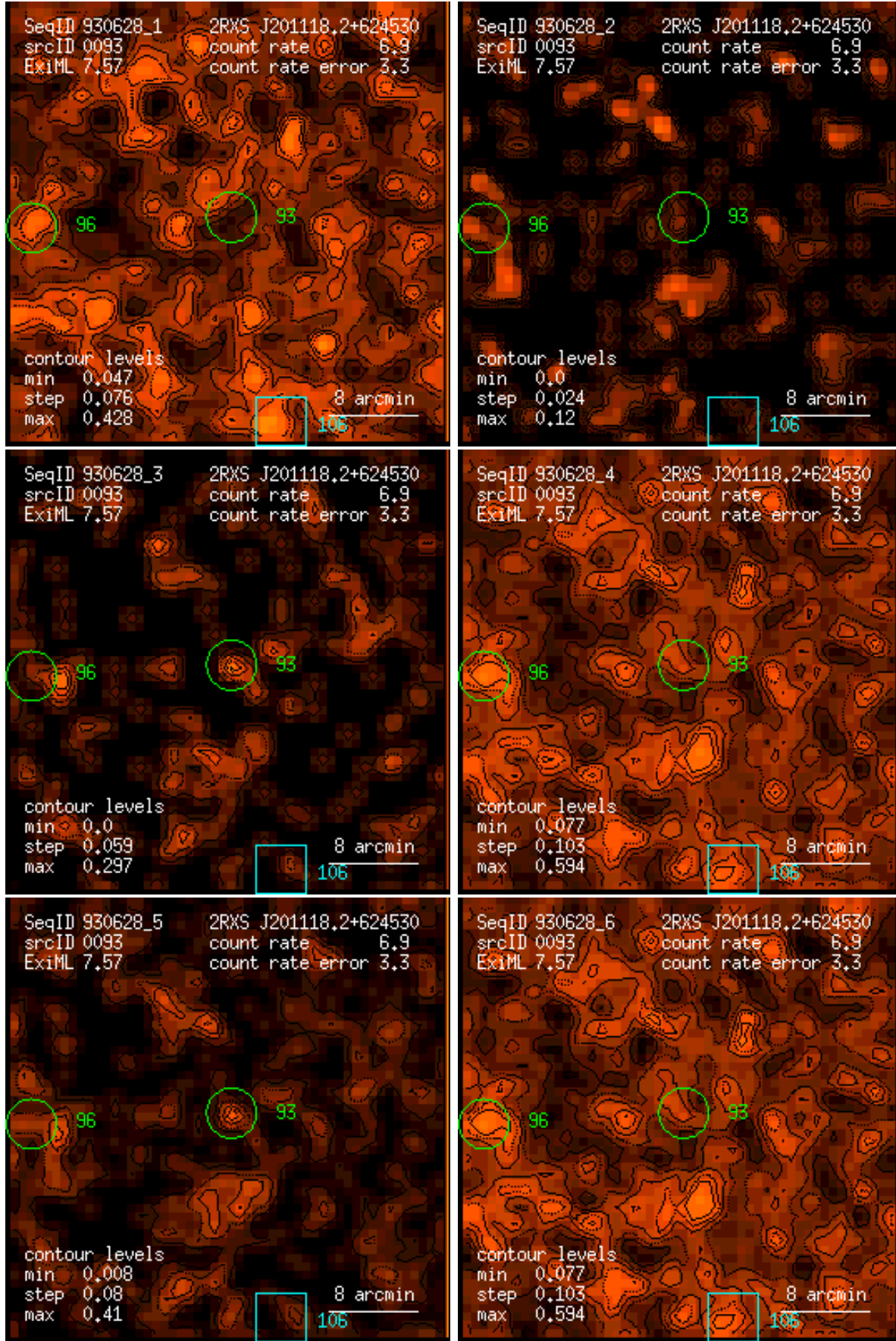
Figure 93: RASS 930628: detection 0093: band rate images, Gaussian filter: (1) PSPC channels 11 – 41, (2) 52 – 90, (3) 91 – 201, (4) 11 – 235, (5) 52 – 201, (6) 11 – 201. Broad band rates in counts/ks. Band rate contour levels in counts/ks/arcmin 2 .
