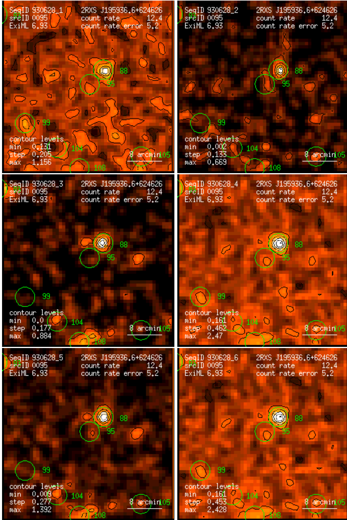
Figure 95: RASS 930628: detection 0095: band rate images, Gaussian filter: (1) PSPC channels 11 – 41, (2) 52 – 90, (3) 91 – 201, (4) 11 – 235, (5) 52 – 201, (6) 11 – 201. Broad band rates in counts/ks. Band rate contour levels in counts/ks/arcmin 2 .
