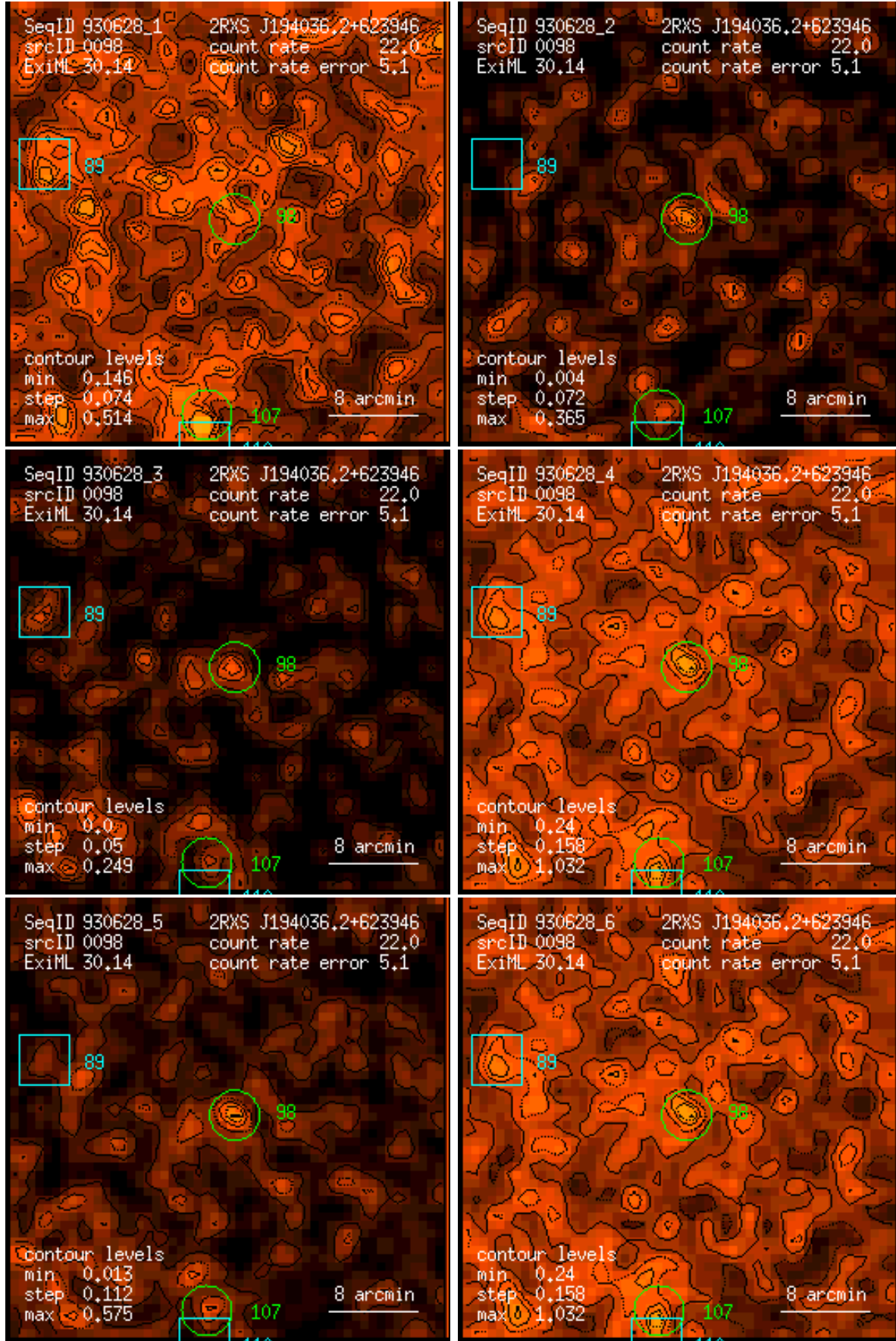
Figure 98: RASS 930628: detection 0098: band rate images, Gaussian filter: (1) PSPC channels 11 – 41, (2) 52 – 90, (3) 91 – 201, (4) 11 – 235, (5) 52 – 201, (6) 11 – 201. Broad band rates in counts/ks. Band rate contour levels in counts/ks/arcmin 2 .
