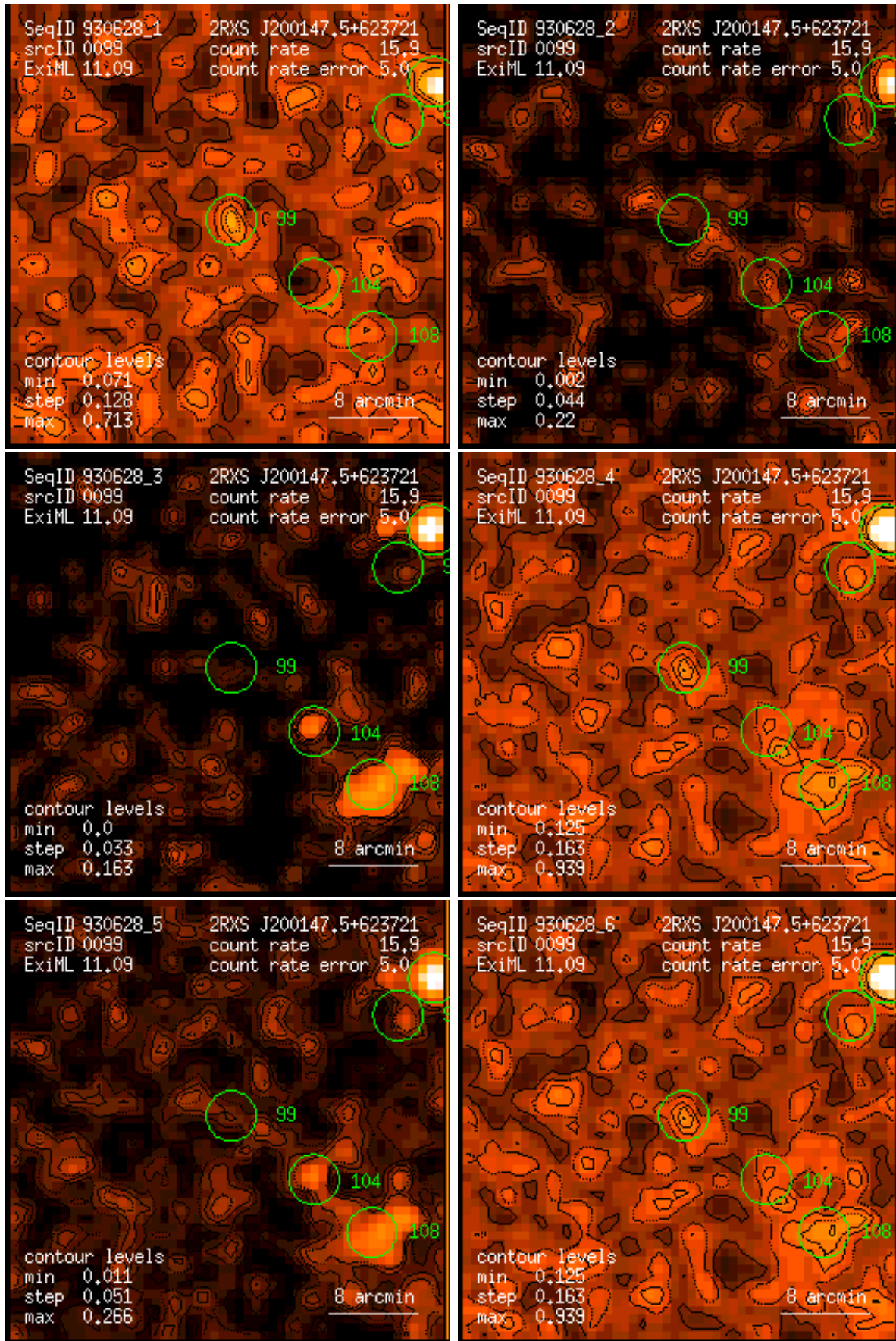
Figure 99: RASS 930628: detection 0099: band rate images, Gaussian filter: (1) PSPC channels 11 – 41, (2) 52 – 90, (3) 91 – 201, (4) 11 – 235, (5) 52 – 201, (6) 11 – 201. Broad band rates in counts/ks. Band rate contour levels in counts/ks/arcmin 2 .
