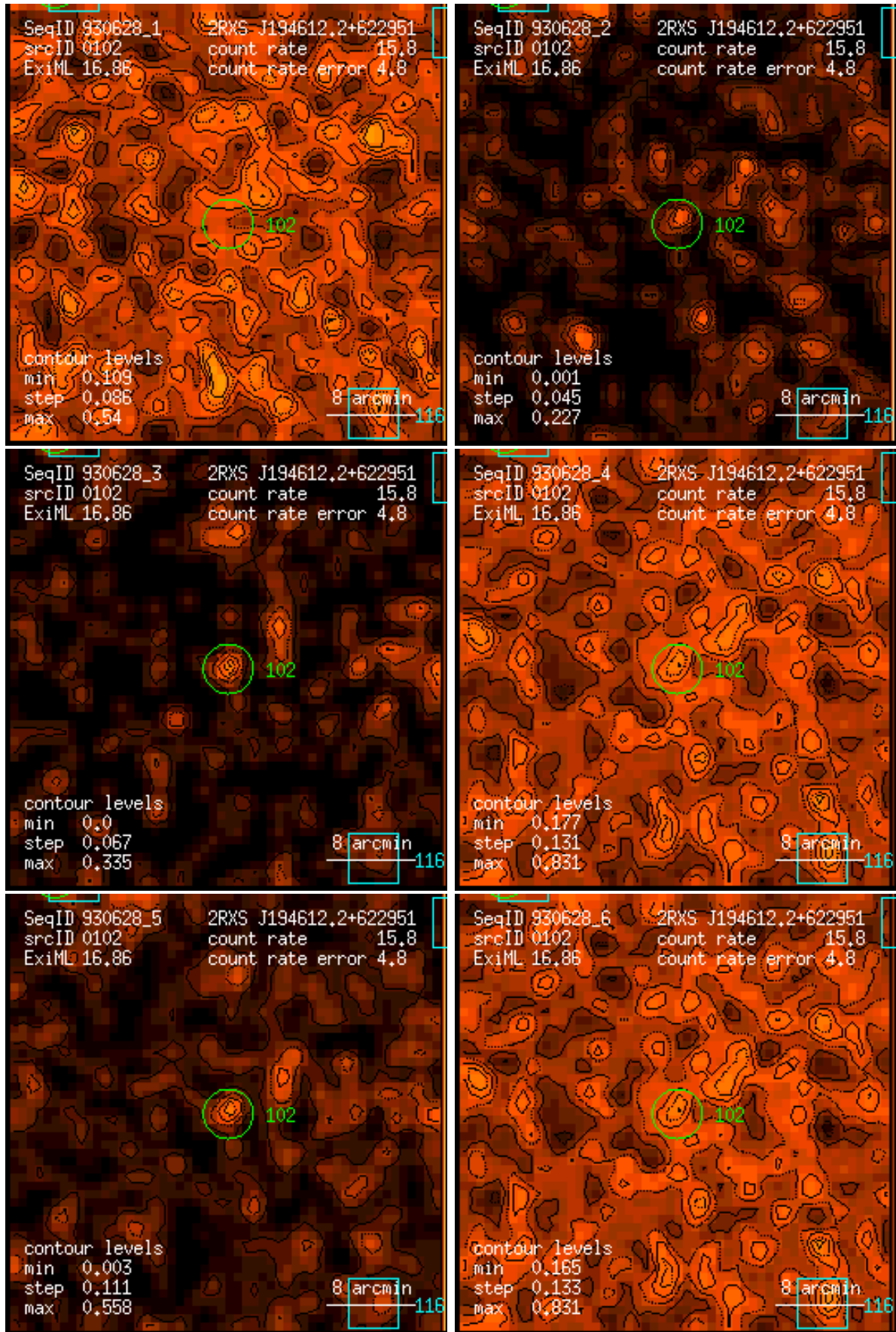
Figure 102: RASS 930628: detection 0102: band rate images, Gaussian filter: (1) PSPC channels 11 – 41, (2) 52 – 90, (3) 91 – 201, (4) 11 – 235, (5) 52 – 201, (6) 11 – 201. Broad band rates in counts/ks. Band rate contour levels in counts/ks/arcmin 2 .
