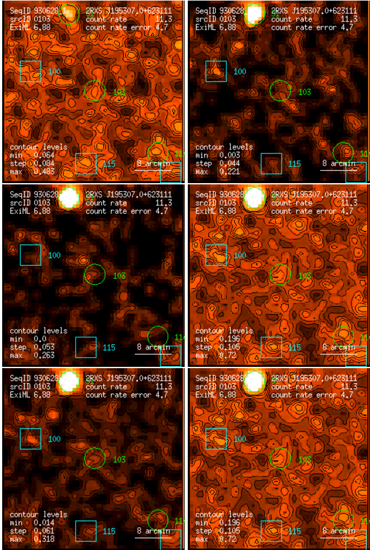
Figure 103: RASS 930628: detection 0103: band rate images, Gaussian filter: (1) PSPPC channels 11 – 41, (2) 52 – 90, (3) 91 – 201, (4) 11 – 235, (5) 52 – 201, (6) 11 – 201. Broad band rates in counts/ks. Band rate contour levels in counts/ks/arcmin 2 .
