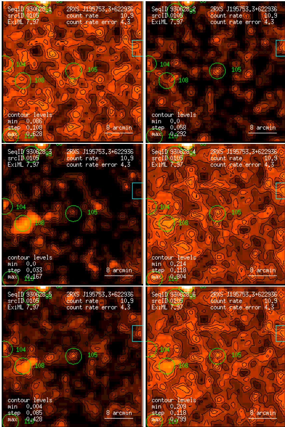
Figure 105: RASS 930628: detection 0105: band rate images, Gaussian filter: (1) PSPC channels 11 – 41, (2) 52 – 90, (3) 91 – 201, (4) 11 – 235, (5) 52 – 201, (6) 11 – 201. Broad band rates in counts/ks. Band rate contour levels in counts/ks/arcmin 2 .
