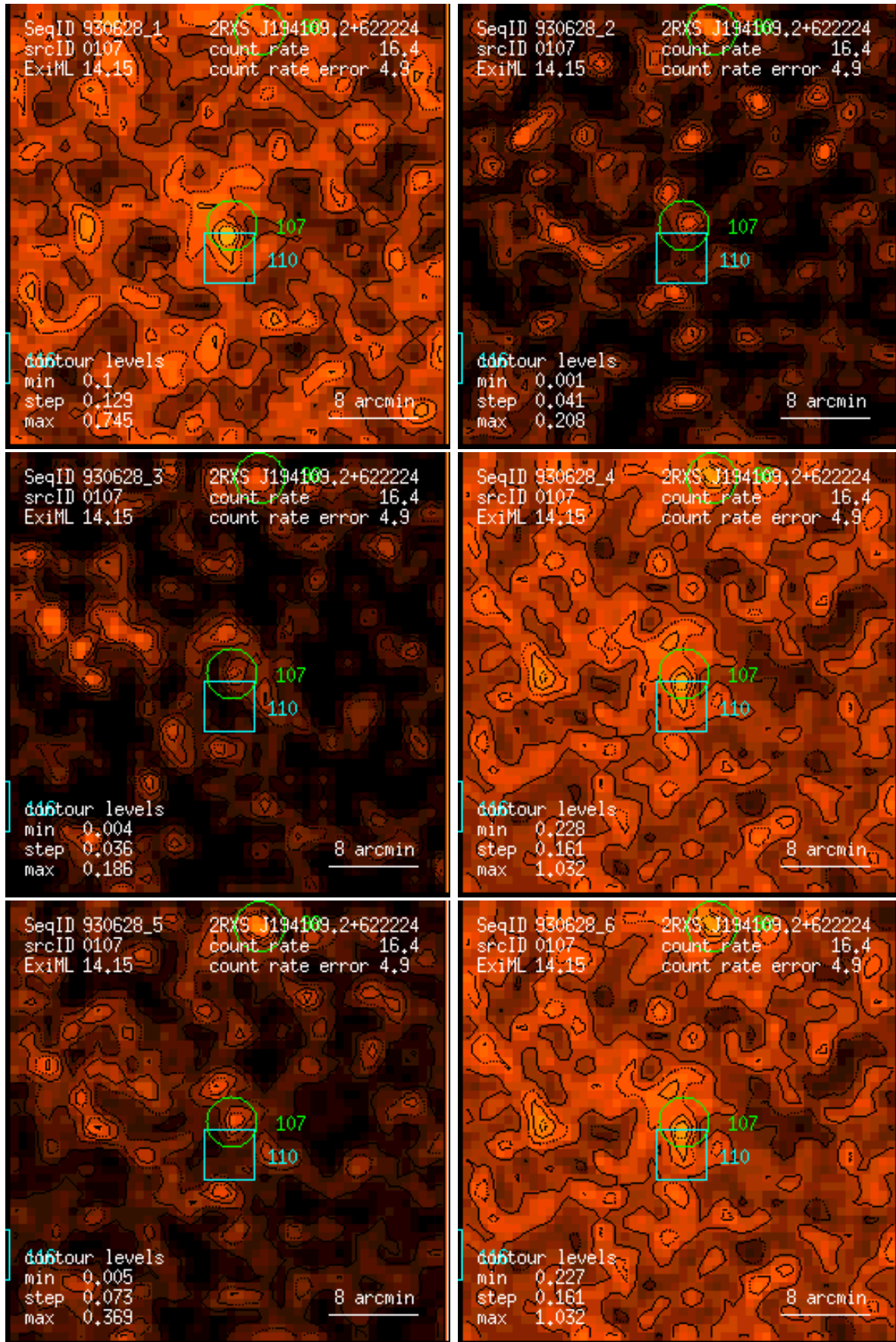
Figure 107: RASS 930628: detection 0107: band rate images, Gaussian filter: (1) PSPC channels 11 – 41, (2) 52 – 90, (3) 91 – 201, (4) 11 – 235, (5) 52 – 201, (6) 11 – 201. Broad band rates in counts/ks. Band rate contour levels in counts/ks/arcmin 2 .
