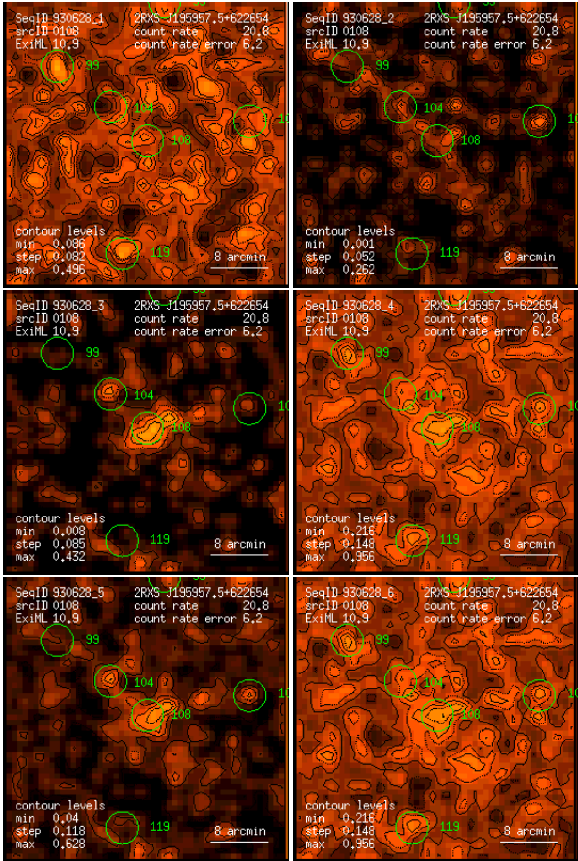
Figure 108: RASS 930628: detection 0108: band rate images, Gaussian filter: (1) PSPC channels 11 – 41, (2) 52 – 90, (3) 91 – 201, (4) 11 – 235, (5) 52 – 201, (6) 11 – 201. Broad band rates in counts/ks. Band rate contour levels in counts/ks/arcmin 2 .
