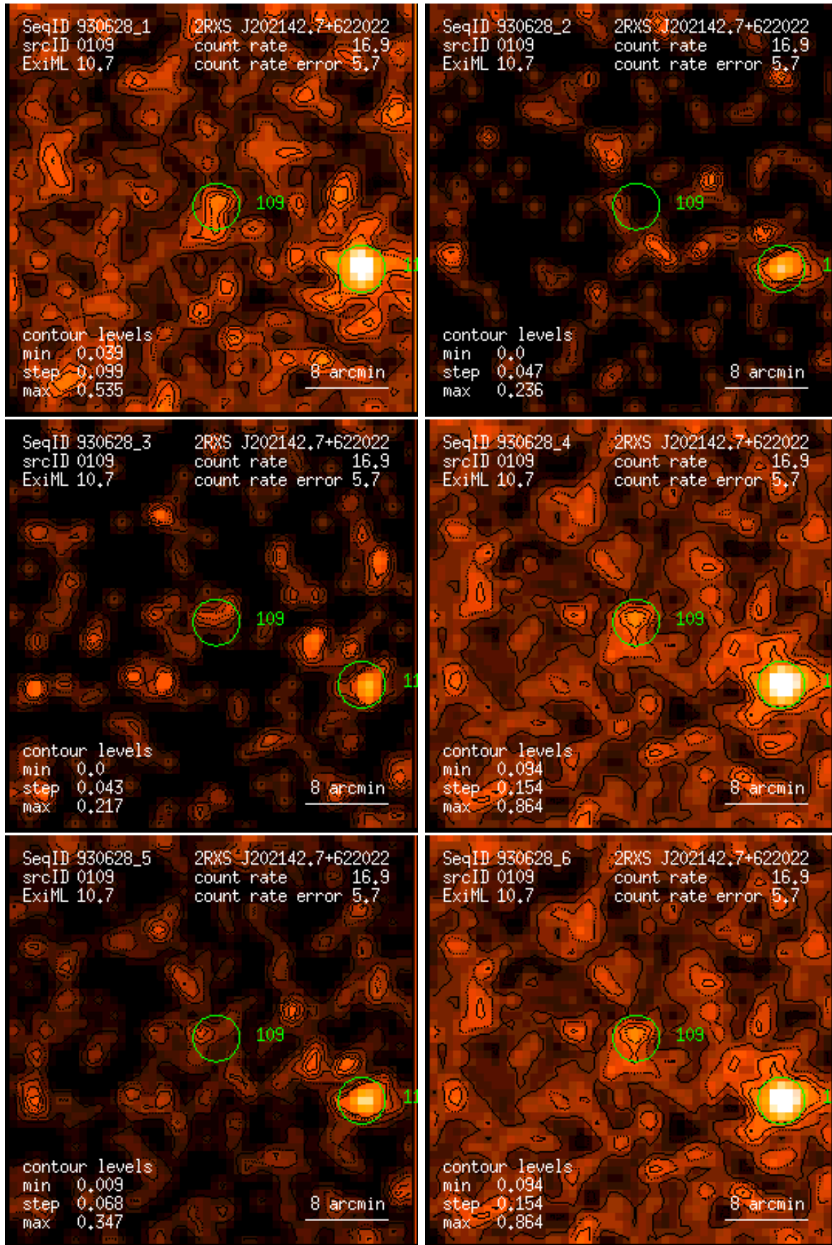
Figure 109: RASS 930628: detection 0109: band rate images, Gaussian filter: (1) PSPC channels 11 – 41, (2) 52 – 90, (3) 91 – 201, (4) 11 – 235, (5) 52 – 201, (6) 11 – 201. Broad band rates in counts/ks. Band rate contour levels in counts/ks/arcmin 2 .
