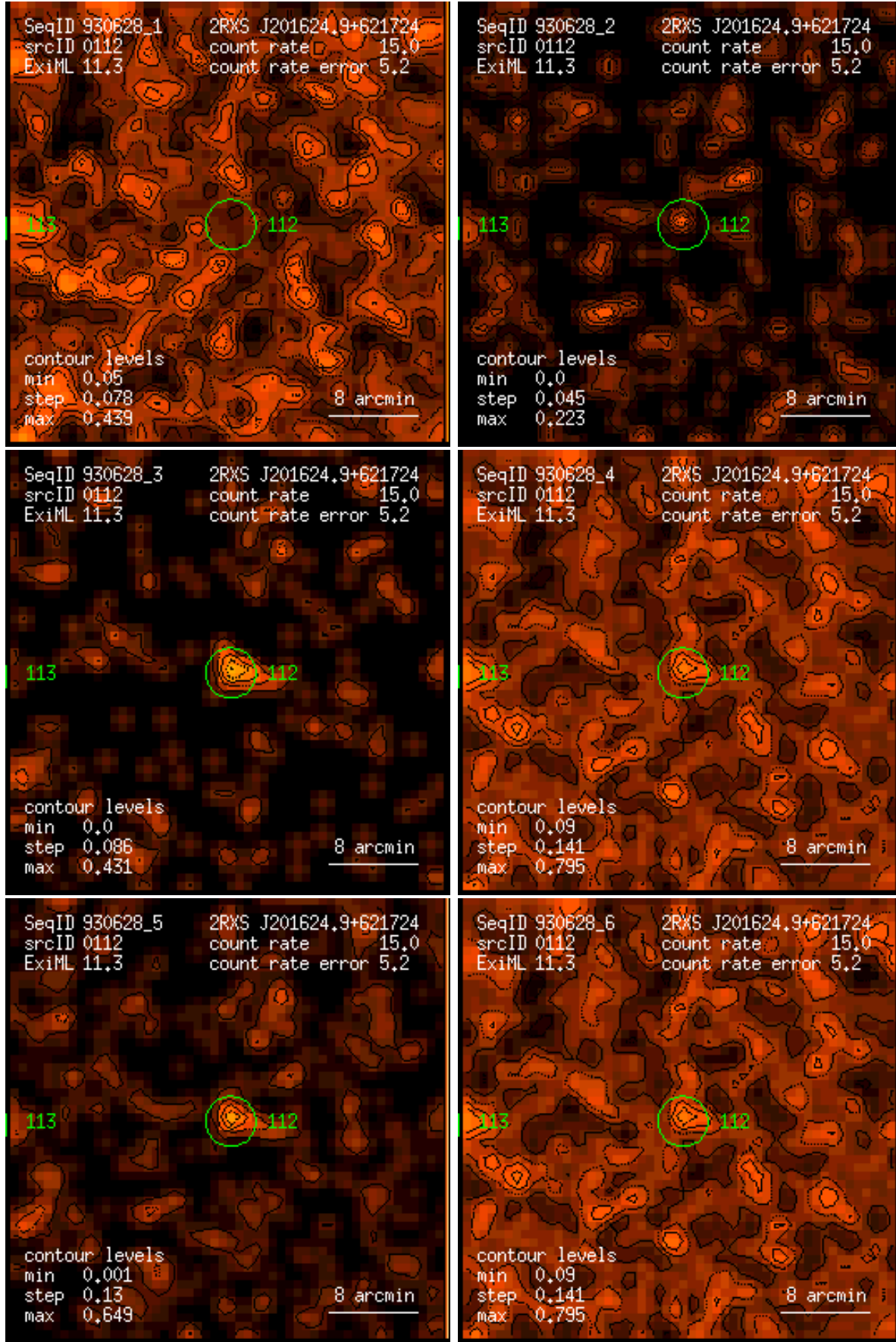
Figure 112: RASS 930628: detection 0112: band rate images, Gaussian filter: (1) PSPC channels 11 – 41, (2) 52 – 90, (3) 91 – 201, (4) 11 – 235, (5) 52 – 201, (6) 11 – 201. Broad band rates in counts/ks. Band rate contour levels in counts/ks/arcmin 2 .
