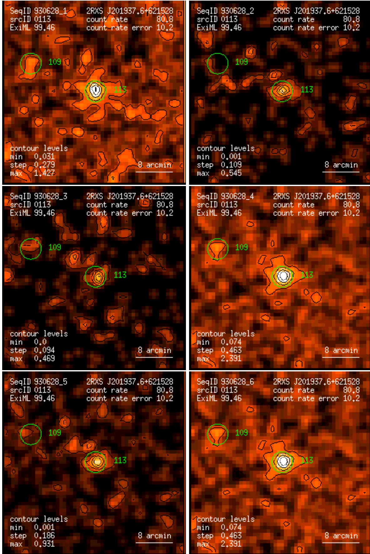
Figure 113: RASS 930628: detection 0113: band rate images, Gaussian filter: (1) PSPC channels 11 – 41, (2) 52 – 90, (3) 91 – 201, (4) 11 – 235, (5) 52 – 201, (6) 11 – 201. Broad band rates in counts/ks. Band rate contour levels in counts/ks/arcmin 2 .
