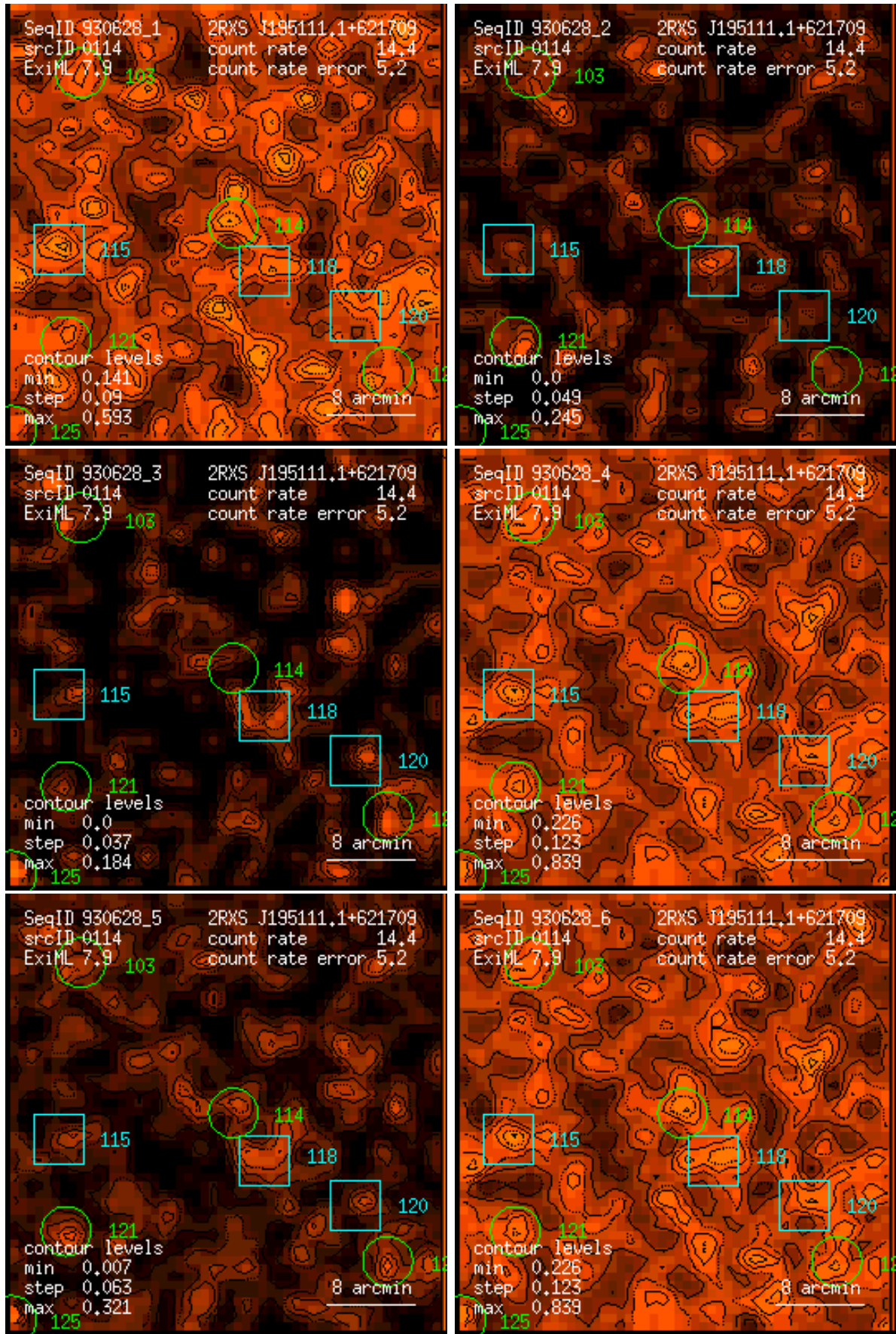
Figure 114: RASS 930628: detection 0114: band rate images, Gaussian filter: (1) PSPC channels 11 – 41, (2) 52 – 90, (3) 91 – 201, (4) 11 – 235, (5) 52 – 201, (6) 11 – 201. Broad band rates in counts/ks. Band rate contour levels in counts/ks/arcmin 2 .
