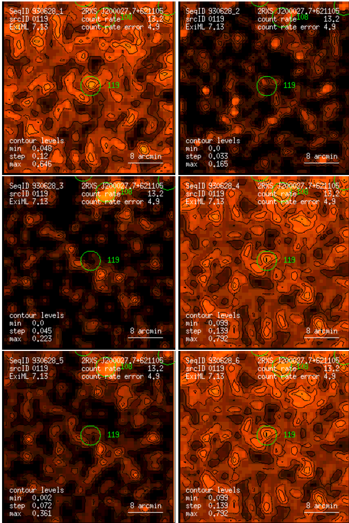
Figure 119: RASS 930628: detection 0119: band rate images, Gaussian filter: (1) PSPC channels 11 – 41, (2) 52 – 90, (3) 91 – 201, (4) 11 – 235, (5) 52 – 201, (6) 11 – 201. Broad band rates in counts/ks. Band rate contour levels in counts/ks/arcmin 2 .
