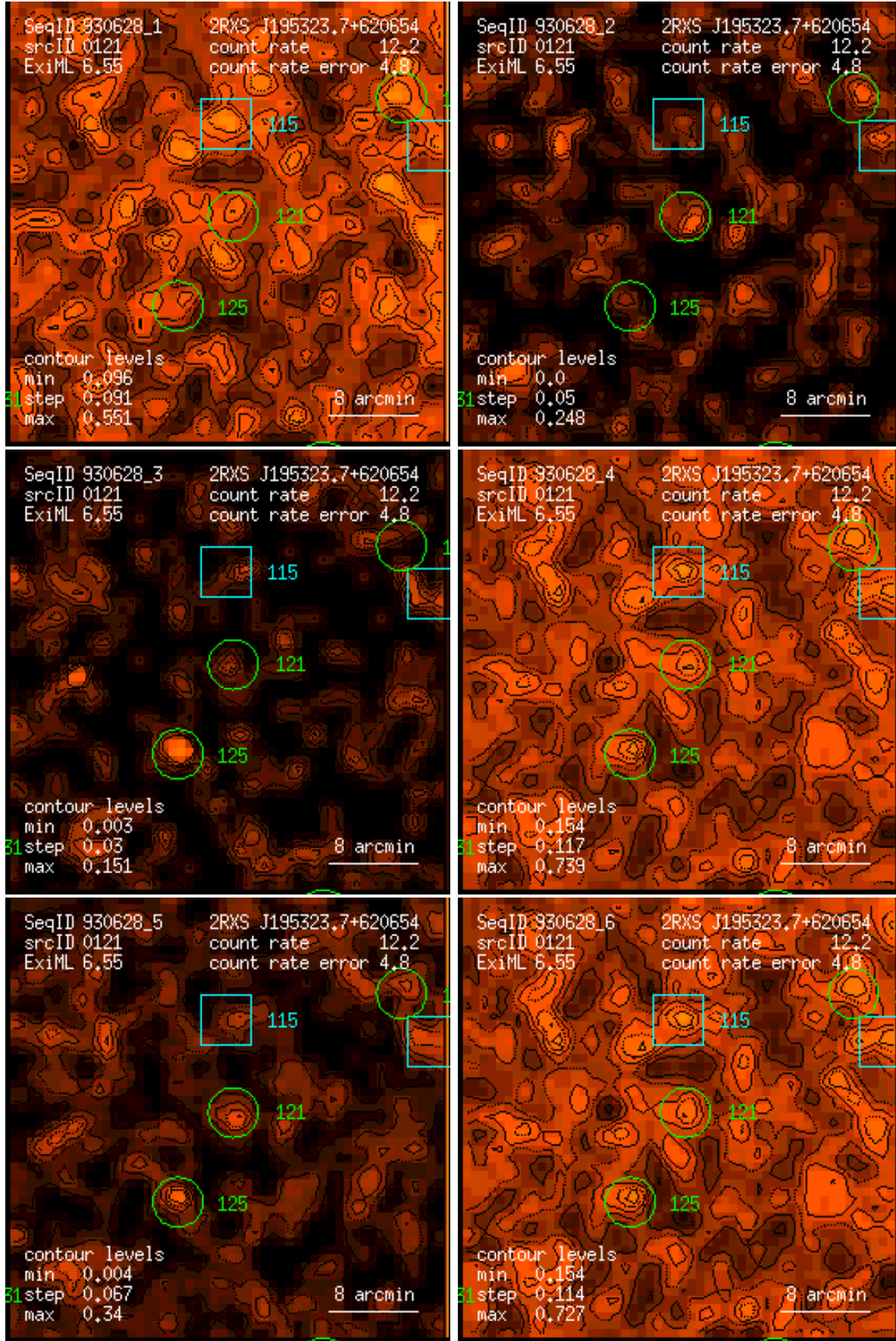
Figure 121: RASS 930628: detection 0121: band rate images, Gaussian filter: (1) PSPC channels 11 – 41, (2) 52 – 90, (3) 91 – 201, (4) 11 – 235, (5) 52 – 201, (6) 11 – 201. Broad band rates in counts/ks. Band rate contour levels in counts/ks/arcmin 2 .
