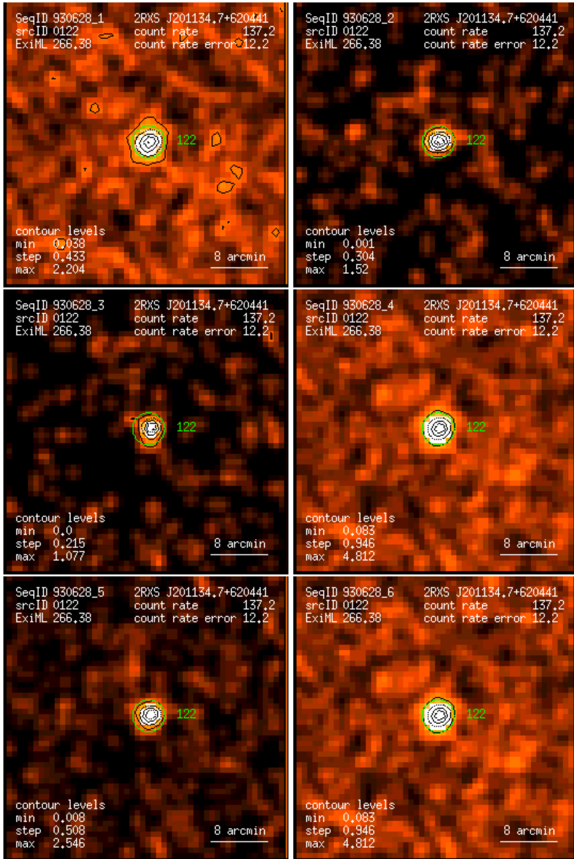
Figure 122: RASS 930628: detection 0122: band rate images, Gaussian filter: (1) PSPC channels 11 – 41, (2) 52 – 90, (3) 91 – 201, (4) 11 – 235, (5) 52 – 201, (6) 11 – 201. Broad band rates in counts/ks. Band rate contour levels in counts/ks/arcmin 2 .
