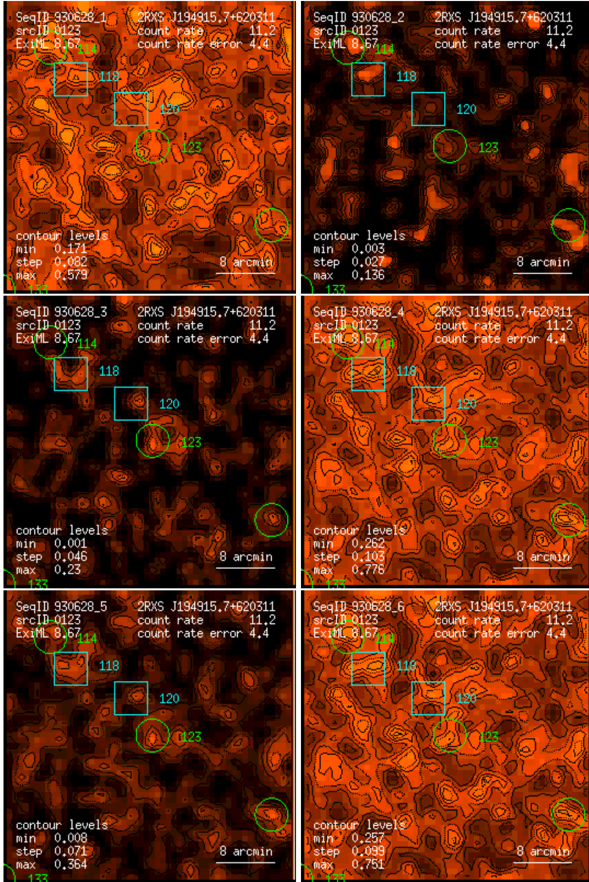
Figure 123: RASS 930628: detection 0123: band rate images, Gaussian filter: (1) PSPC channels 11 – 41, (2) 52 – 90, (3) 91 – 201, (4) 11 – 235, (5) 52 – 201, (6) 11 – 201. Broad band rates in counts/ks. Band rate contour levels in counts/ks/arcmin 2 .
