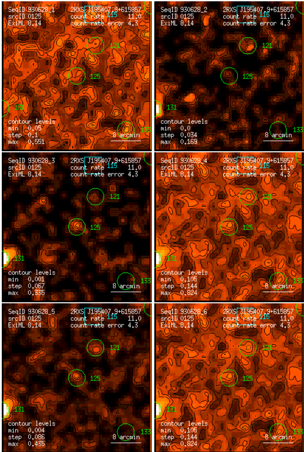
Figure 125: RASS 930628: detection 0125: band rate images, Gaussian filter: (1) PSPC channels 11 – 41, (2) 52 – 90, (3) 91 – 201, (4) 11 – 235, (5) 52 – 201, (6) 11 – 201. Broad band rates in counts/ks. Band rate contour levels in counts/ks/arcmin 2 .
