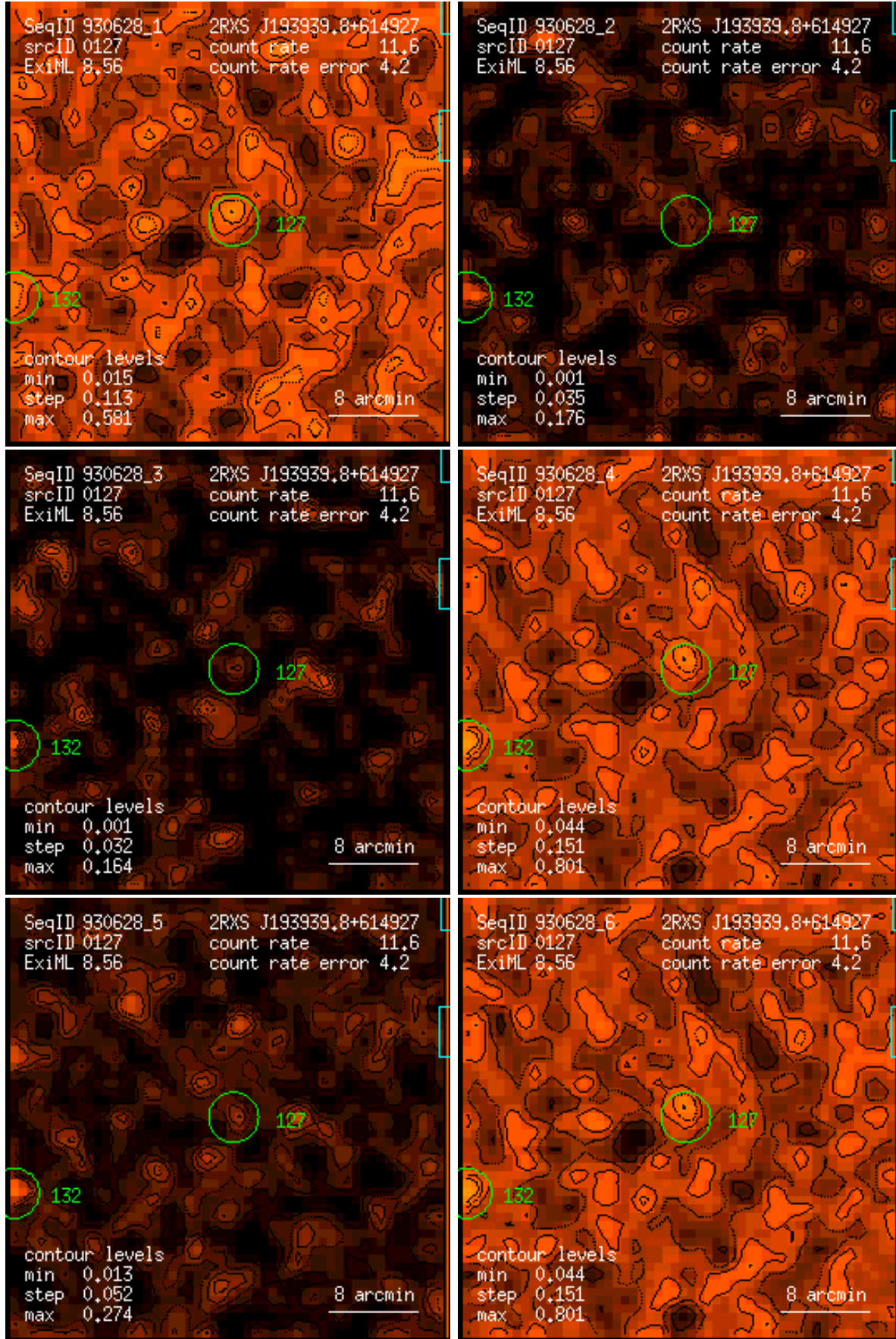
Figure 127: RASS 930628: detection 0127: band rate images, Gaussian filter: (1) PSPC channels 11 – 41, (2) 52 – 90, (3) 91 – 201, (4) 11 – 235, (5) 52 – 201, (6) 11 – 201. Broad band rates in counts/ks. Band rate contour levels in counts/ks/arcmin 2 .
