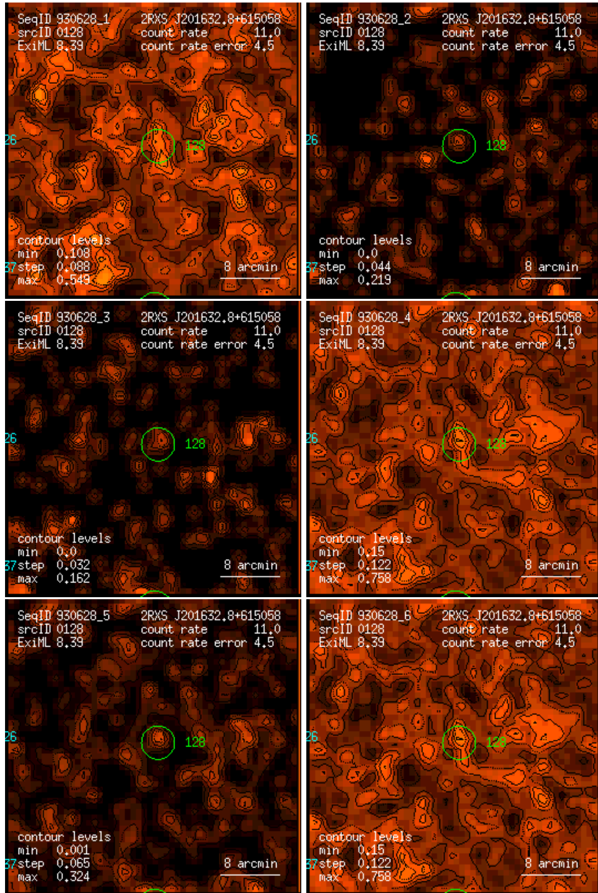
Figure 128: RASS 930628: detection 0128: band rate images, Gaussian filter: (1) PSPC channels 11 – 41, (2) 52 – 90, (3) 91 – 201, (4) 11 – 235, (5) 52 – 201, (6) 11 – 201. Broad band rates in counts/ks. Band rate contour levels in counts/ks/arcmin 2 .
