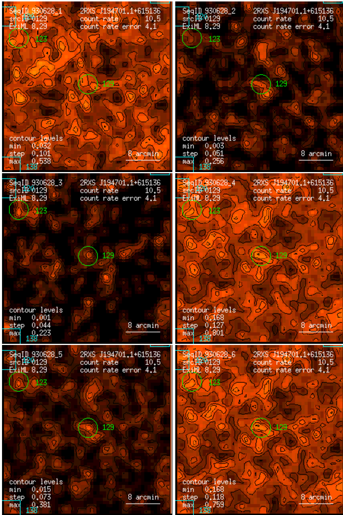
Figure 129: RASS 930628: detection 0129: band rate images, Gaussian filter: (1) PSPC channels 11 – 41, (2) 52 – 90, (3) 91 – 201, (4) 11 – 235, (5) 52 – 201, (6) 11 – 201. Broad band rates in counts/ks. Band rate contour levels in counts/ks/arcmin 2 .
