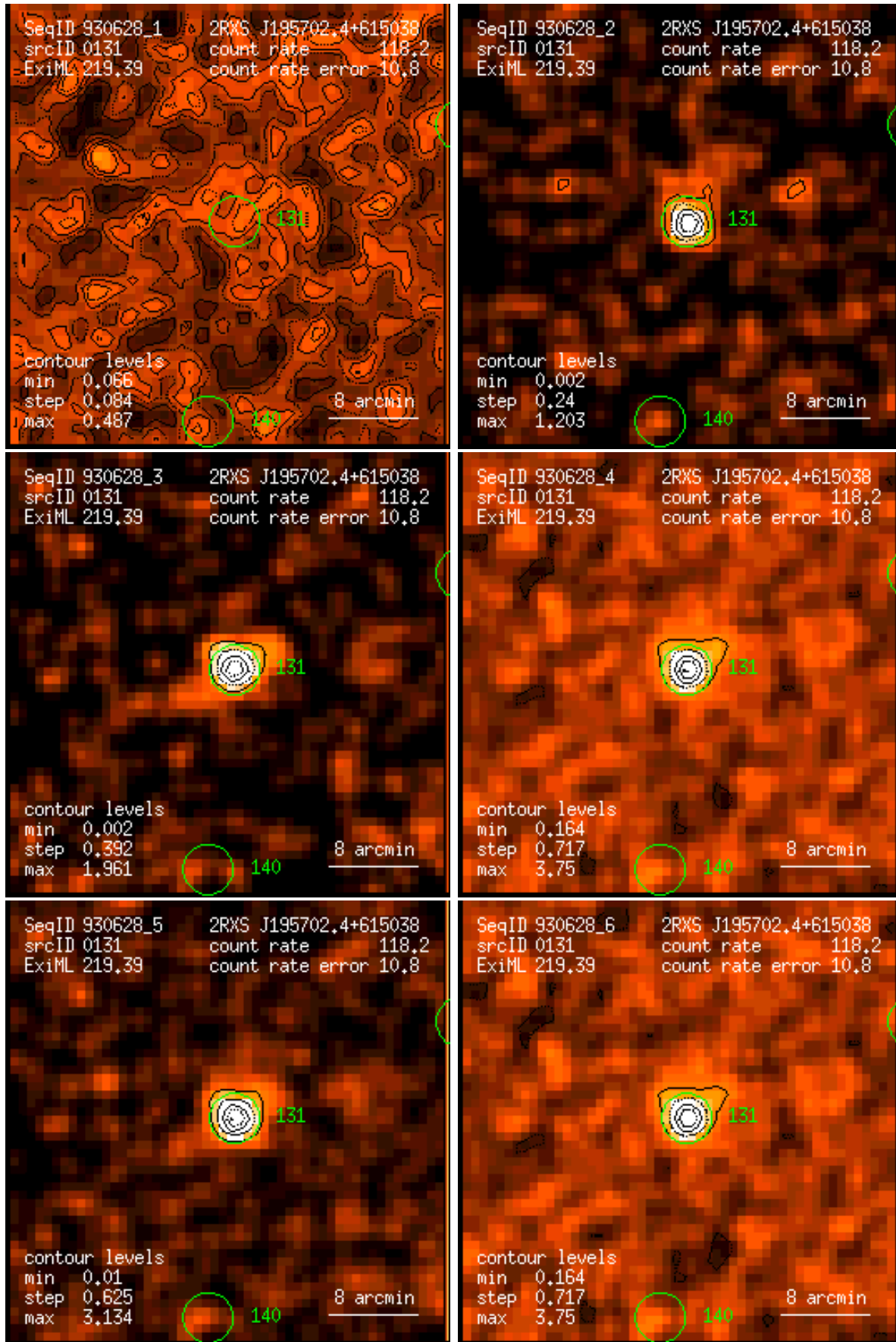
Figure 131: RASS 930628: detection 0131: band rate images, Gaussian filter: (1) PSPC channels 11 – 41, (2) 52 – 90, (3) 91 – 201, (4) 11 – 235, (5) 52 – 201, (6) 11 – 201. Broad band rates in counts/ks. Band rate contour levels in counts/ks/arcmin 2 .
