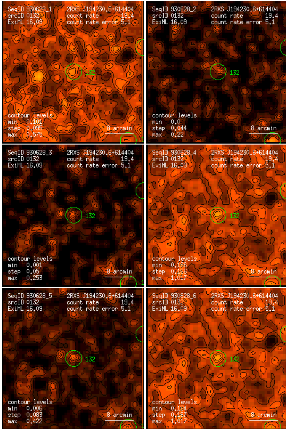
Figure 132: RASS 930628: detection 0132: band rate images, Gaussian filter: (1) PSPC channels 11 – 41, (2) 52 – 90, (3) 91 – 201, (4) 11 – 235, (5) 52 – 201, (6) 11 – 201. Broad band rates in counts/ks. Band rate contour levels in counts/ks/arcmin 2 .
